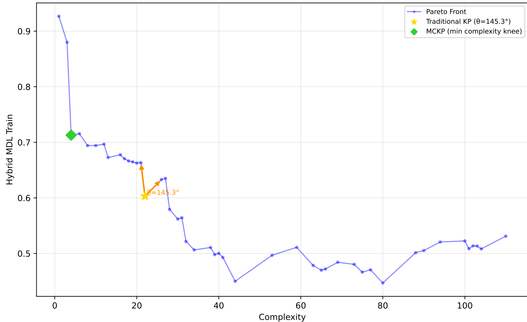
589_fri_c2_1000_25 - Run 16 - SVP - Hybrid MDL Train \lambda_1=0.10, \lambda_2=0.00, \lambda_3=0.10 | Difficulty: 1.00 | Method: hmr
