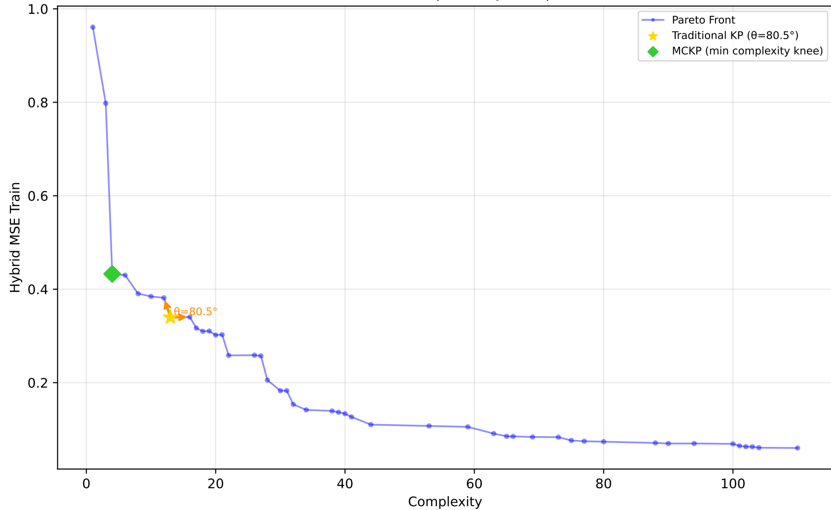
589_fri_c2_1000_25 - Run 16 - SVP - Hybrid MSE Train \lambda_1=0.10, \bar{\lambda}_2=0.00, \bar{\lambda}_3=0.10 | Difficulty: 1.00 | Method: hmr
