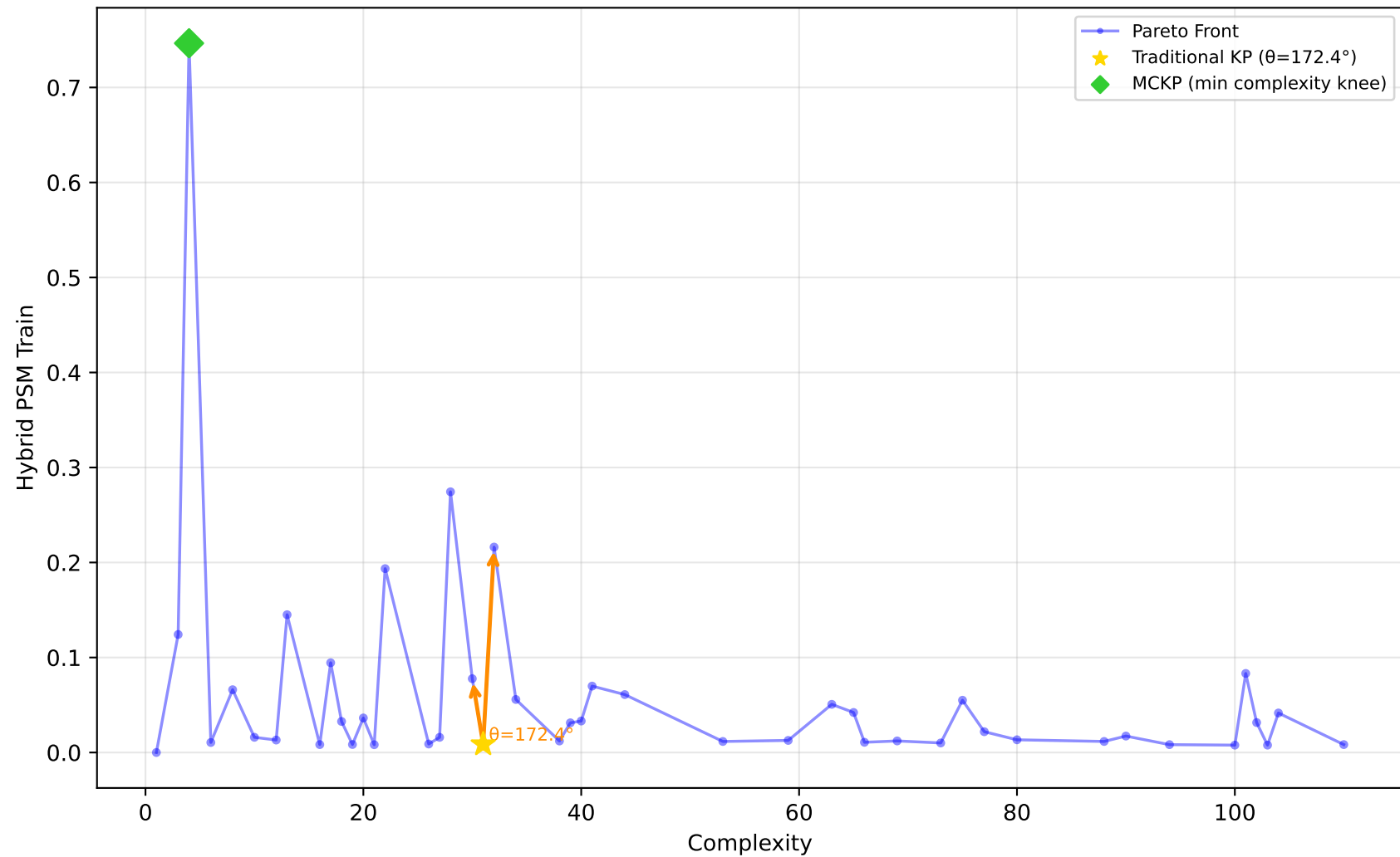
589_fri_c2_1000_25 - Run 16 - SVP - Hybrid PSM Train \lambda_1=0.10, \bar{\lambda}_2=0.00, \bar{\lambda}_3=0.10 | Difficulty: 1.00 | Method: hmr
