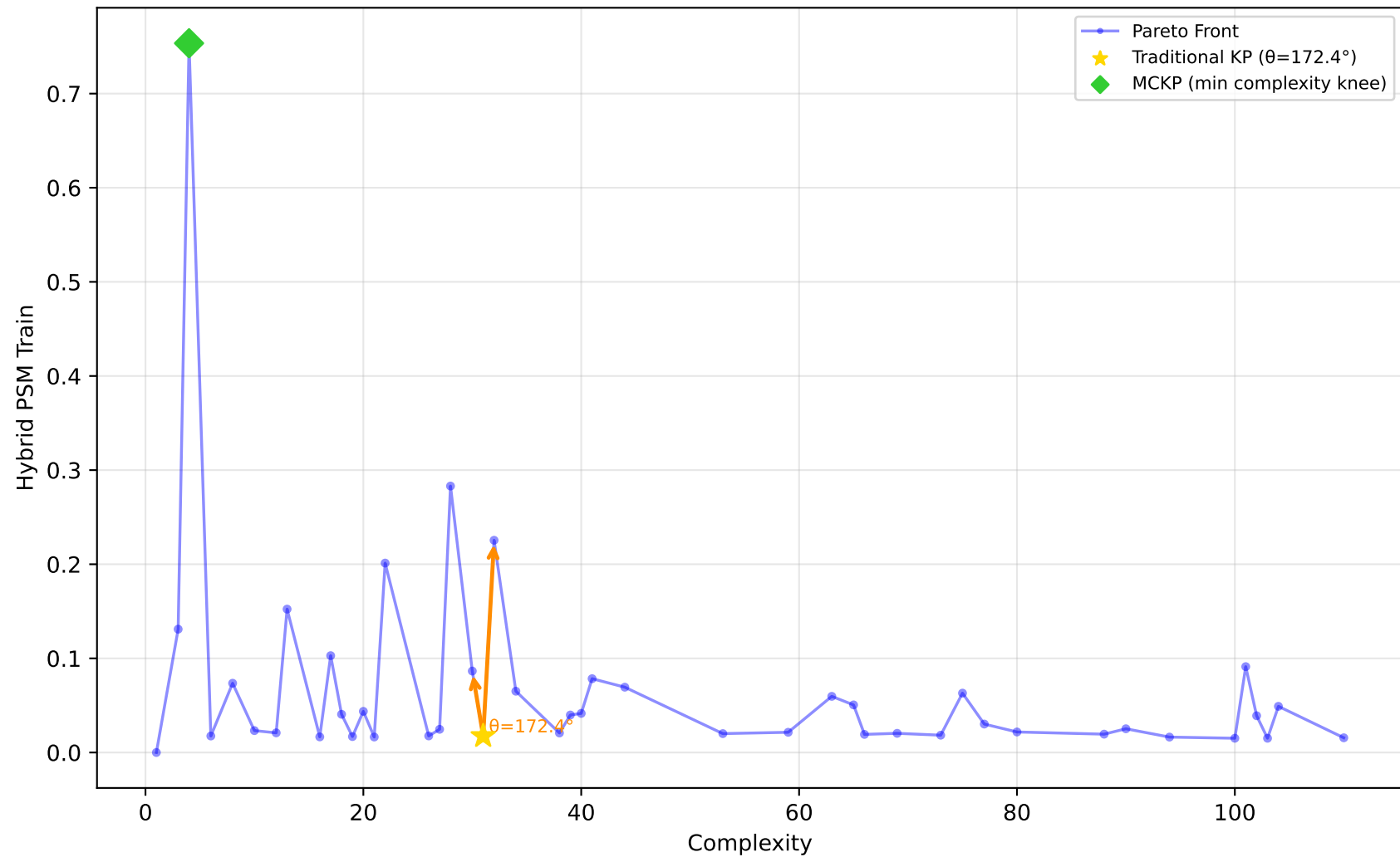
589_fri_c2_1000_25 - Run 16 - SVP - Hybrid PSM Train \lambda_1=0.20, \bar{\lambda}_2=0.00, \bar{\lambda}_3=1.00 | Difficulty: 1.00 | Method: hmr
