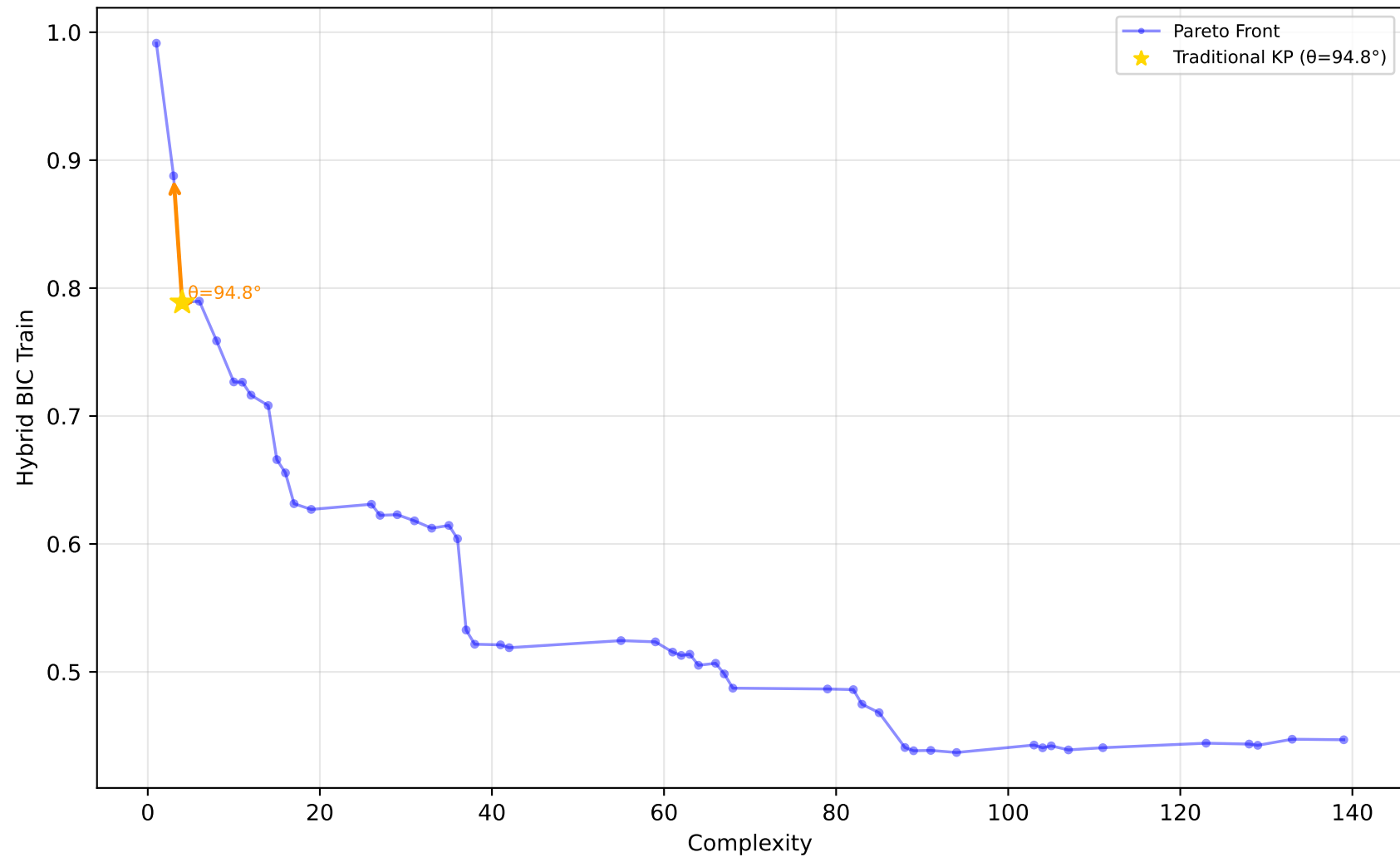
589_fri_c2_1000_25 - Run 17 - MVP - Hybrid BIC Train \lambda_1=0.00, \bar{\lambda}_2=0.00, \bar{\lambda}_3=0.00 | Difficulty: 1.00 | Method: hmr
