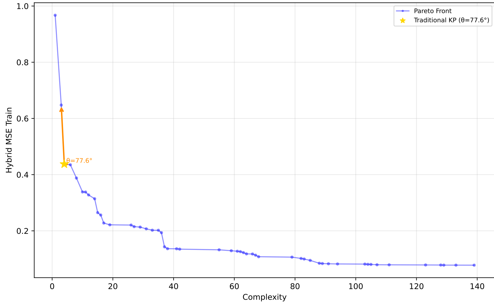
589_fri_c2_1000_25 - Run 17 - MVP - Hybrid MSE Train \lambda_1=0.00, \lambda_2=0.00, \lambda_3=0.00 | Difficulty: 1.00 | Method: hmr
