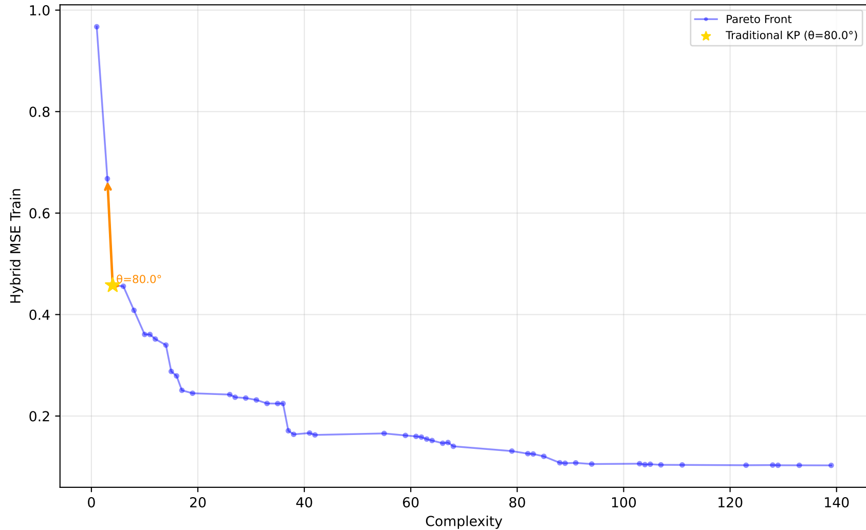
589_fri_c2_1000_25 - Run 17 - MVP - Hybrid MSE Train \lambda_1=0.30, \lambda_2=0.00, \lambda_3=0.20 | Difficulty: 1.00 | Method: hmr
