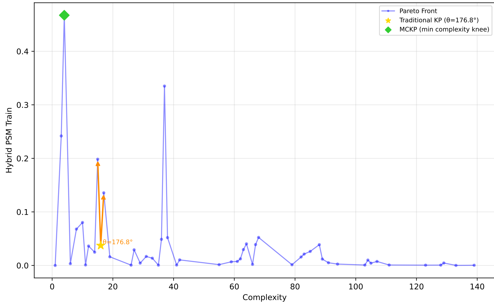
589_fri_c2_1000_25 - Run 17 - MVP - Hybrid PSM Train \lambda_1=0.00, \lambda_2=0.00, \lambda_3=0.00 | Difficulty: 1.00 | Method: hmr
