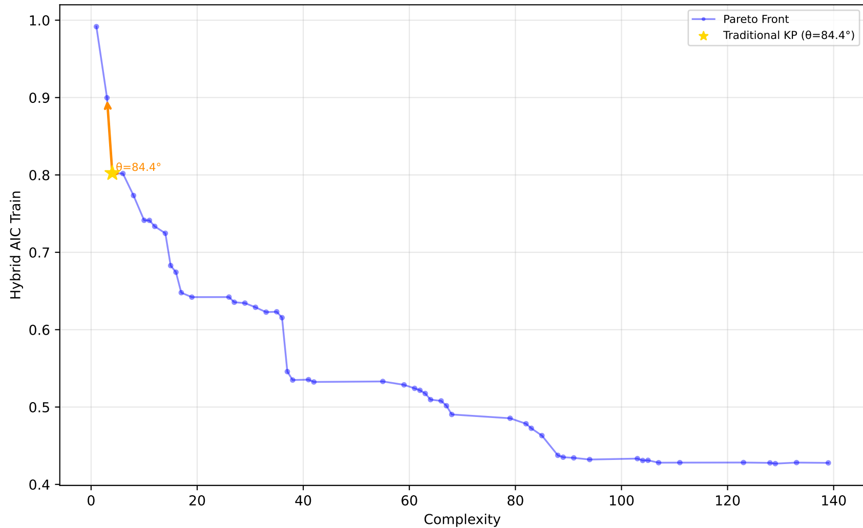
589_fri_c2_1000_25 - Run 17 - SVP - Hybrid AIC Train \lambda_1=0.10, \bar{\lambda}_2=0.00, \bar{\lambda}_3=0.10 | Difficulty: 1.00 | Method: hmr
