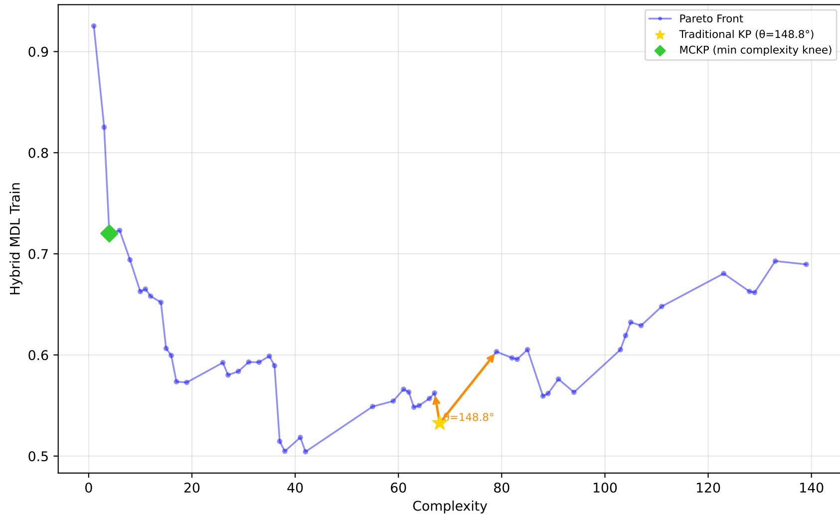
589_fri_c2_1000_25 - Run 17 - SVP - Hybrid MDL Train \lambda_1=0.10, \lambda_2=0.00, \lambda_3=0.10 | Difficulty: 1.00 | Method: hmr
