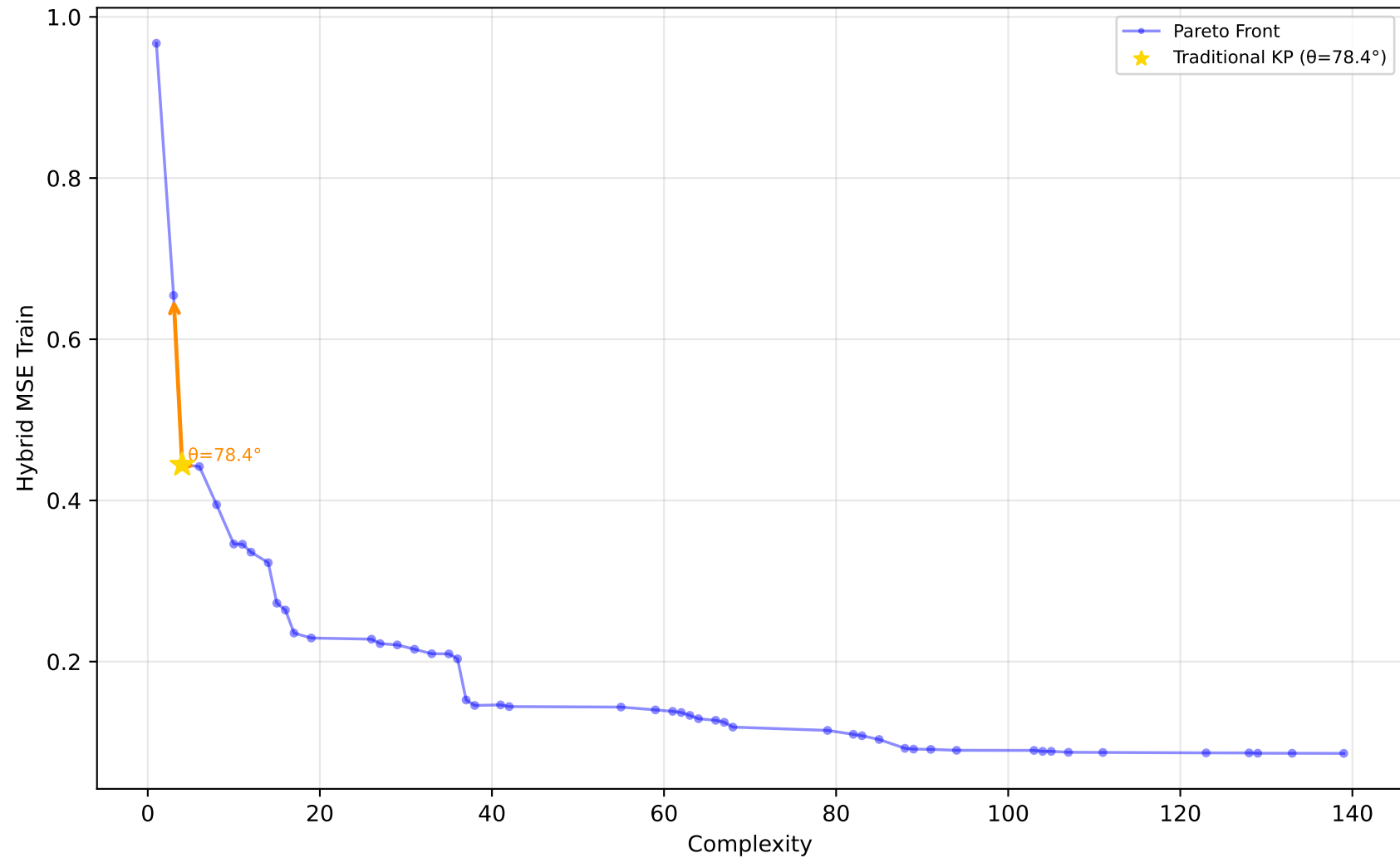
589_fri_c2_1000_25 - Run 17 - SVP - Hybrid MSE Train \lambda_1=0.10, \bar{\lambda}_2=0.00, \bar{\lambda}_3=0.10 | Difficulty: 1.00 | Method: hmr
