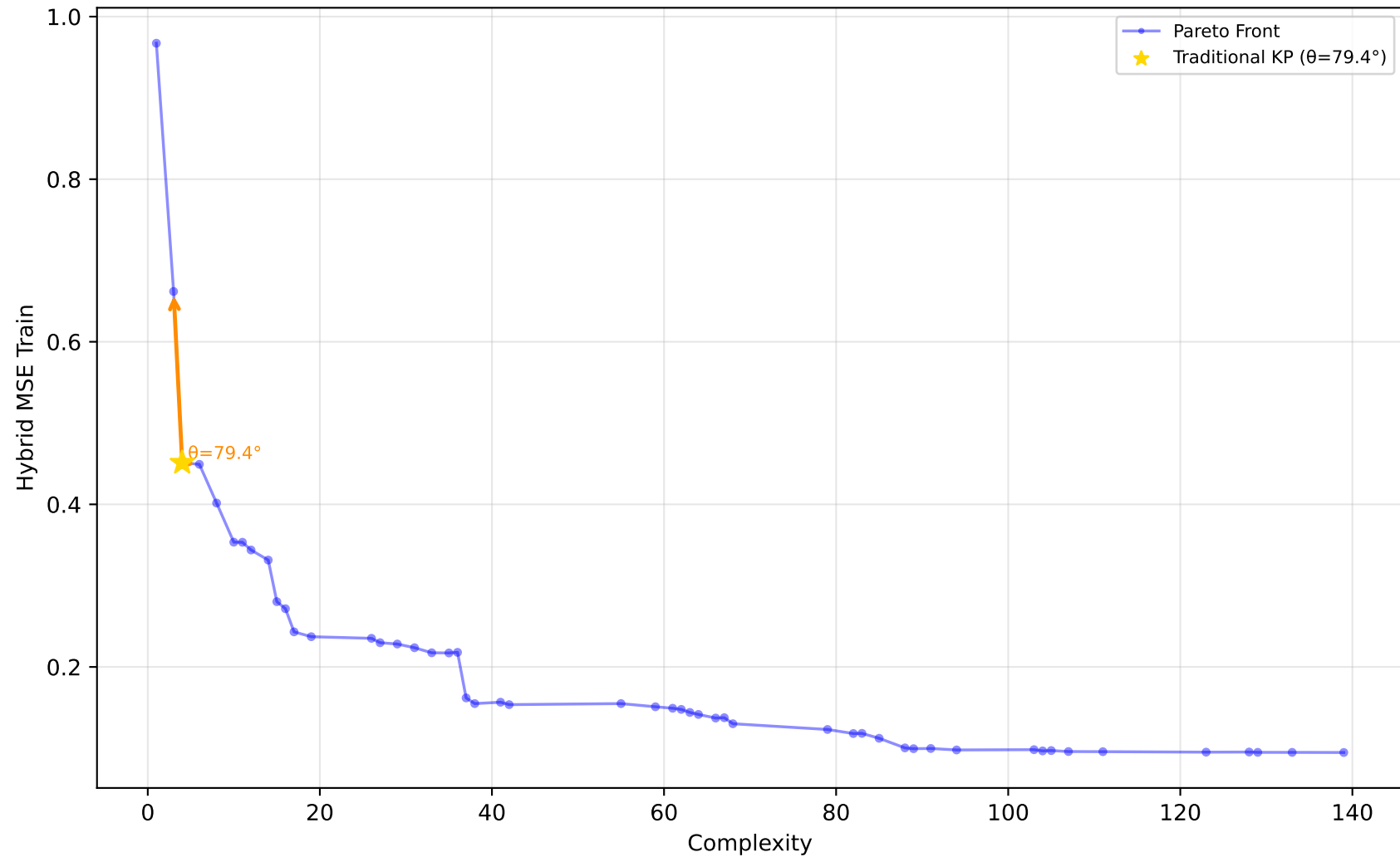
589_fri_c2_1000_25 - Run 17 - SVP - Hybrid MSE Train \lambda_1=0.20, \bar{\lambda}_2=0.00, \bar{\lambda}_3=1.00 | Difficulty: 1.00 | Method: hmr
