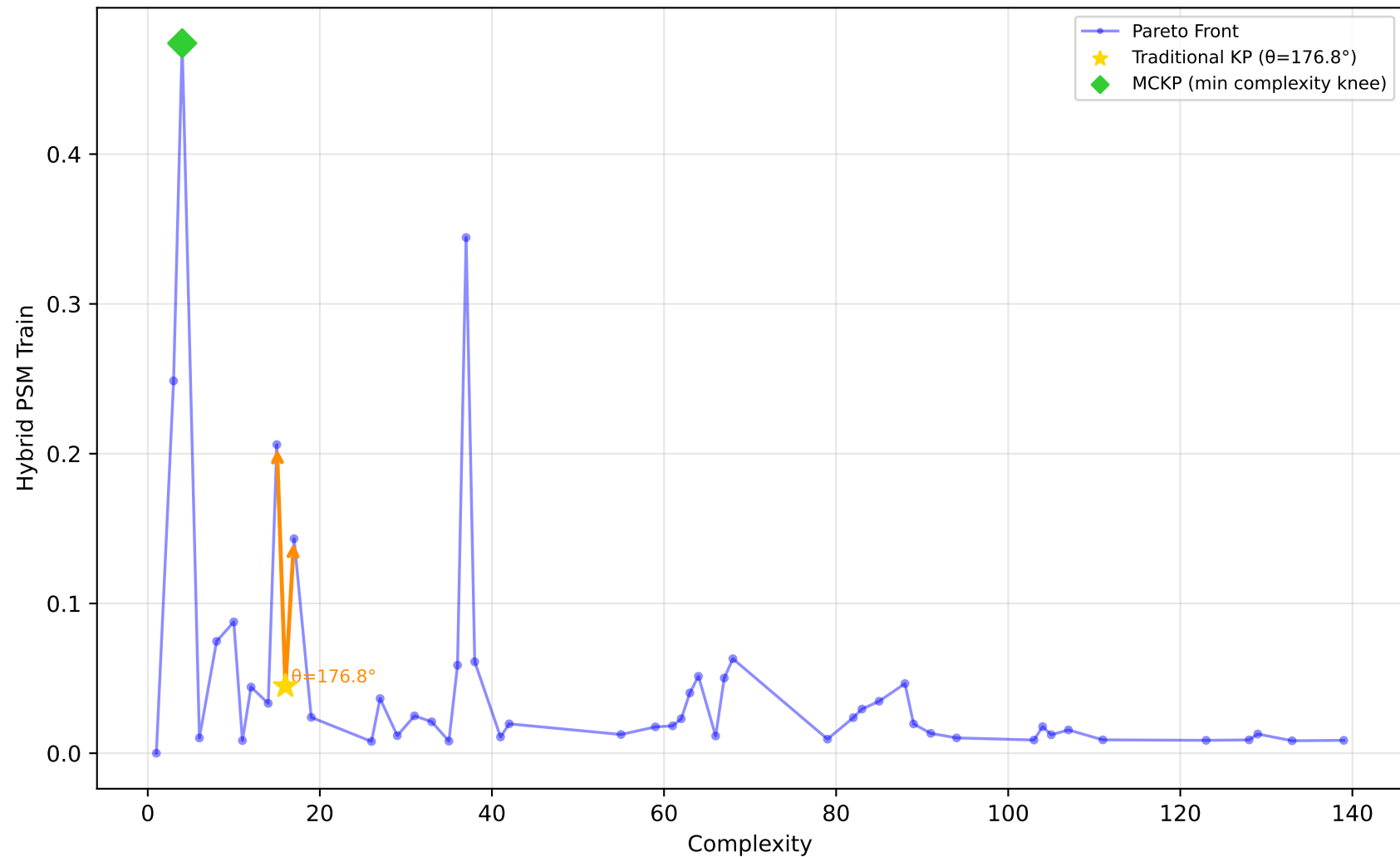
589_fri_c2_1000_25 - Run 17 - SVP - Hybrid PSM Train \lambda_1=0.10, \bar{\lambda}_2=0.00, \bar{\lambda}_3=0.10 | Difficulty: 1.00 | Method: hmr
