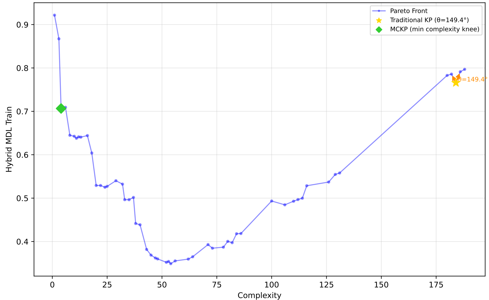
589_fri_c2_1000_25 - Run 18 - MVP - Hybrid MDL Train \lambda_1=0.00, \bar{\lambda}_2=0.00, \bar{\lambda}_3=0.00 | Difficulty: 1.00 | Method: hmr
