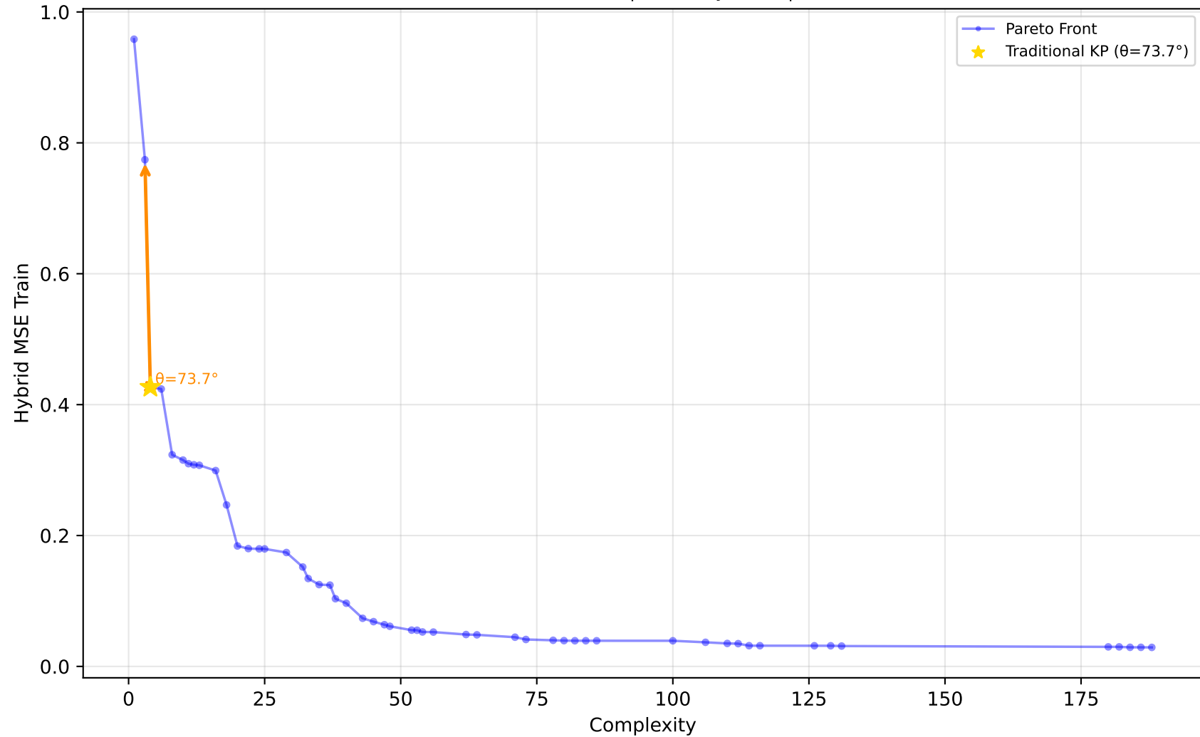
589_fri_c2_1000_25 - Run 18 - MVP - Hybrid MSE Train \lambda_1=0.00, \lambda_2=0.00, \lambda_3=0.00 | Difficulty: 1.00 | Method: hmr
