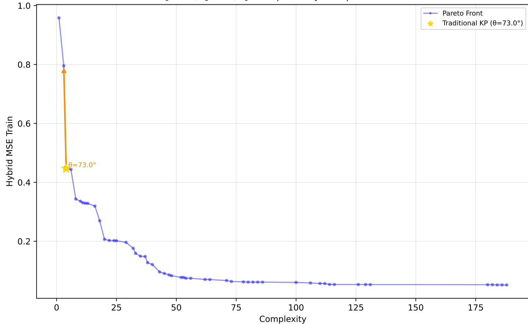
589_fri_c2_1000_25 - Run 18 - MVP - Hybrid MSE Train \lambda_1=0.30, \lambda_2=0.00, \lambda_3=0.20 | Difficulty: 1.00 | Method: hmr
