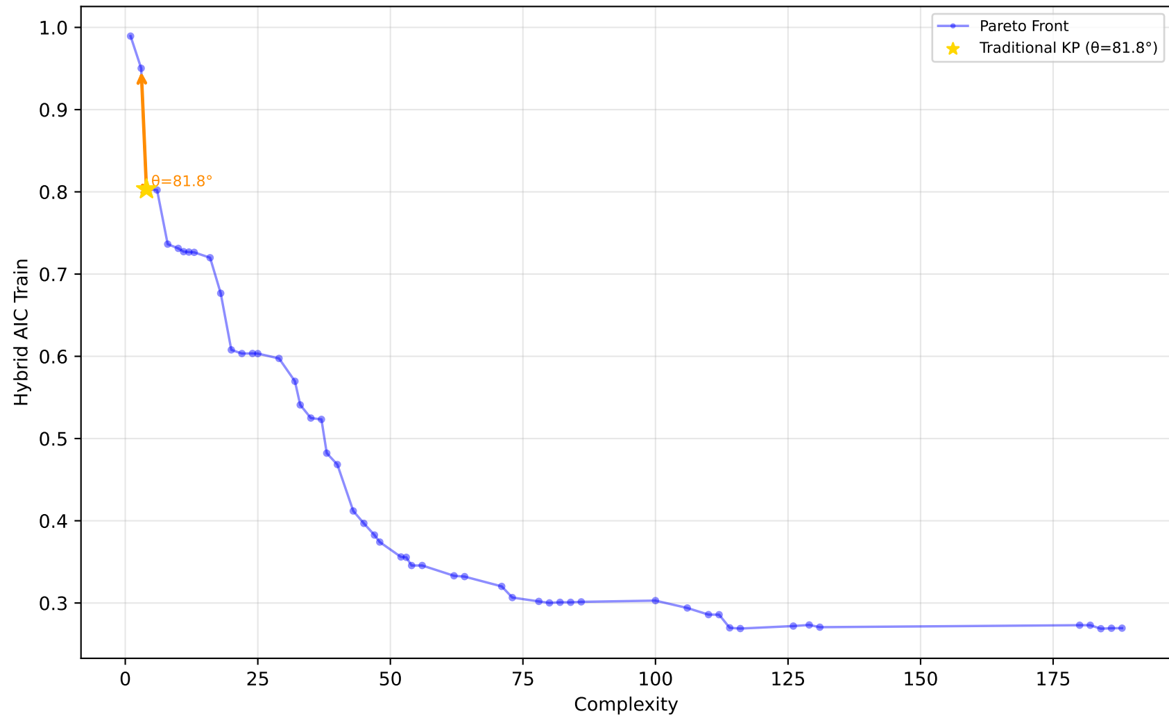
589_fri_c2_1000_25 - Run 18 - SVP - Hybrid AIC Train \lambda_1=0.20, \lambda_2=0.00, \lambda_3=1.00 | Difficulty: 1.00 | Method: hmr
