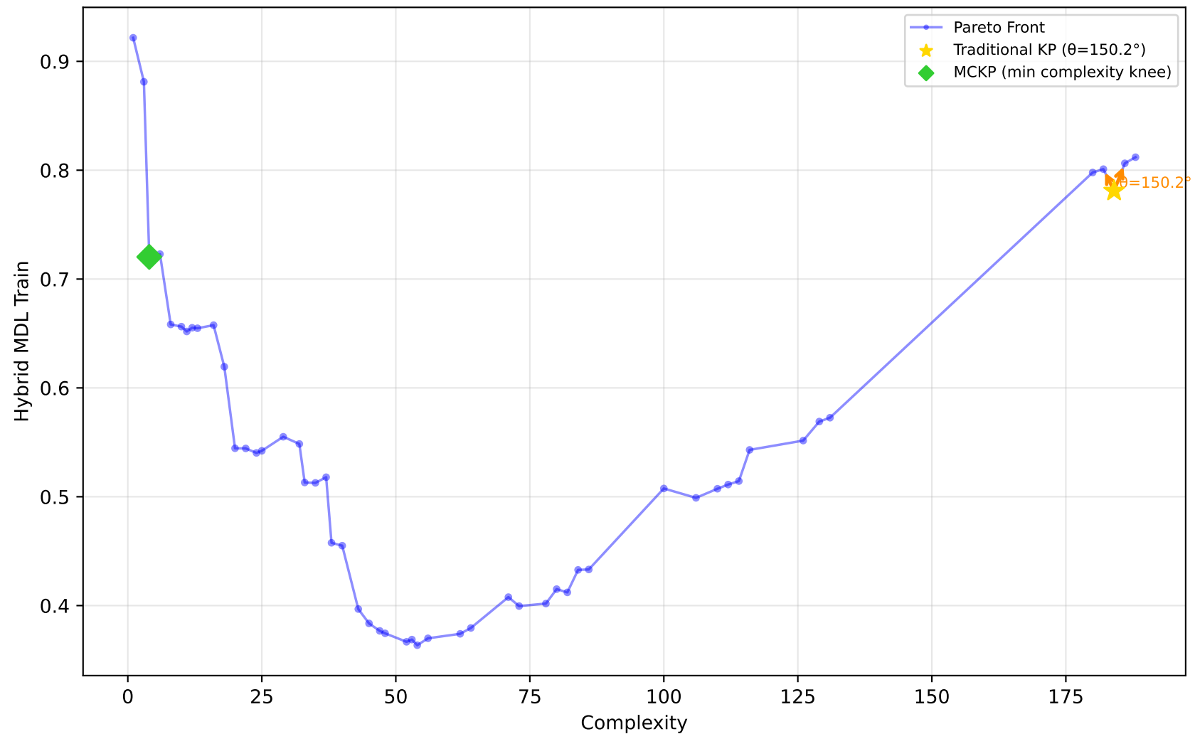
589_fri_c2_1000_25 - Run 18 - SVP - Hybrid MDL Train \lambda_1=0.20, \bar{\lambda}_2=0.00, \bar{\lambda}_3=1.00 | Difficulty: 1.00 | Method: hmr
