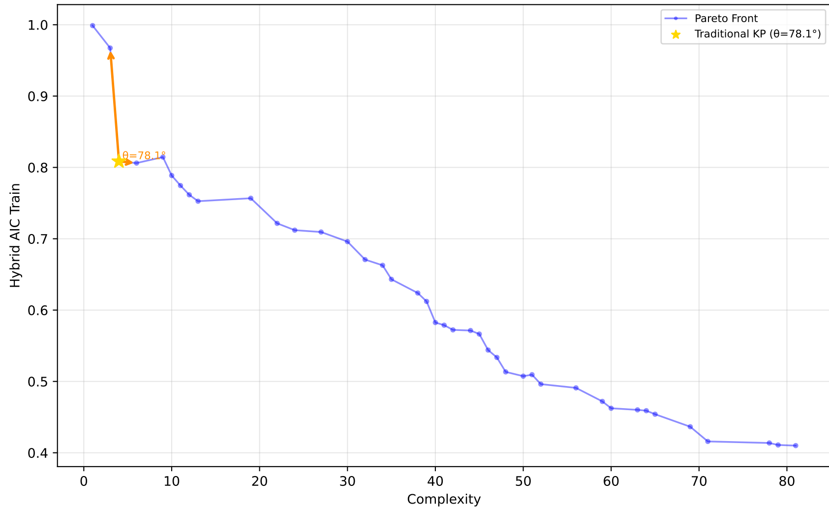
589_fri_c2_1000_25 - Run 19 - MVP - Hybrid AIC Train \lambda_1=0.30, \bar{\lambda}_2=0.00, \bar{\lambda}_3=0.20 | Difficulty: 1.00 | Method: hmr
