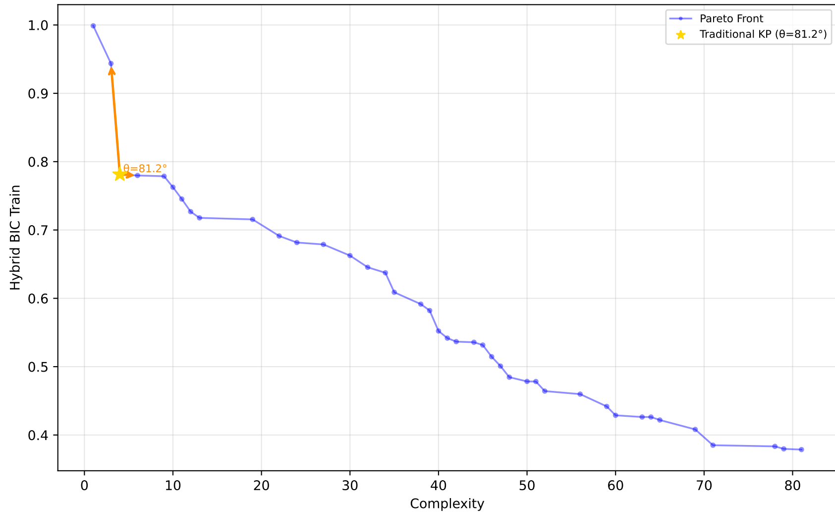
589_fri_c2_1000_25 - Run 19 - MVP - Hybrid BIC Train \lambda_1=0.00, \bar{\lambda}_2=0.00, \bar{\lambda}_3=0.00 | Difficulty: 1.00 | Method: hmr
