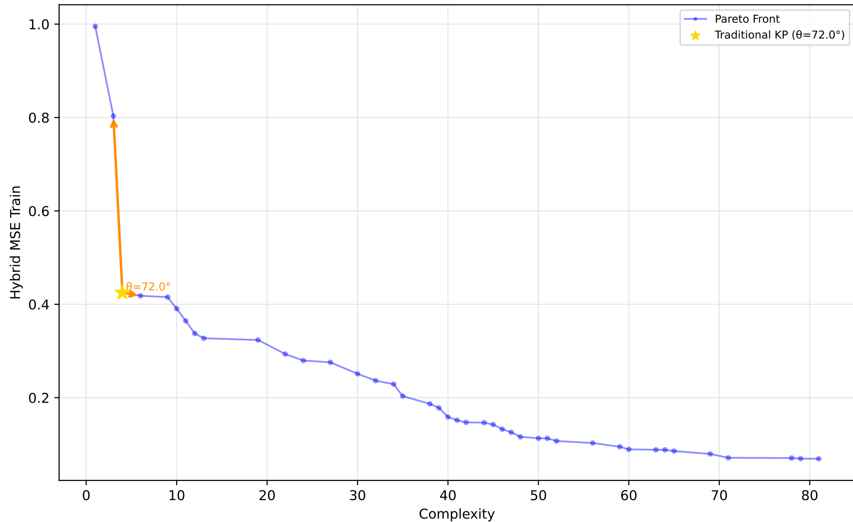
589_fri_c2_1000_25 - Run 19 - MVP - Hybrid MSE Train \lambda_1=0.00, \lambda_2=0.00, \lambda_3=0.00 | Difficulty: 1.00 | Method: hmr
