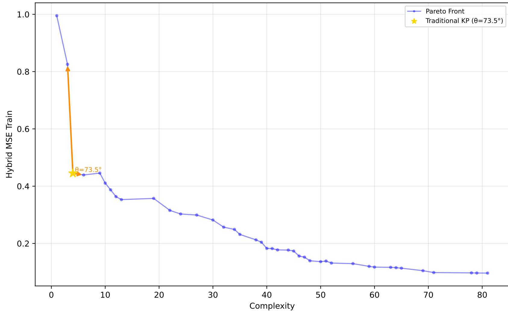
589_fri_c2_1000_25 - Run 19 - MVP - Hybrid MSE Train \lambda_1=0.30, \lambda_2=0.00, \lambda_3=0.20 | Difficulty: 1.00 | Method: hmr
