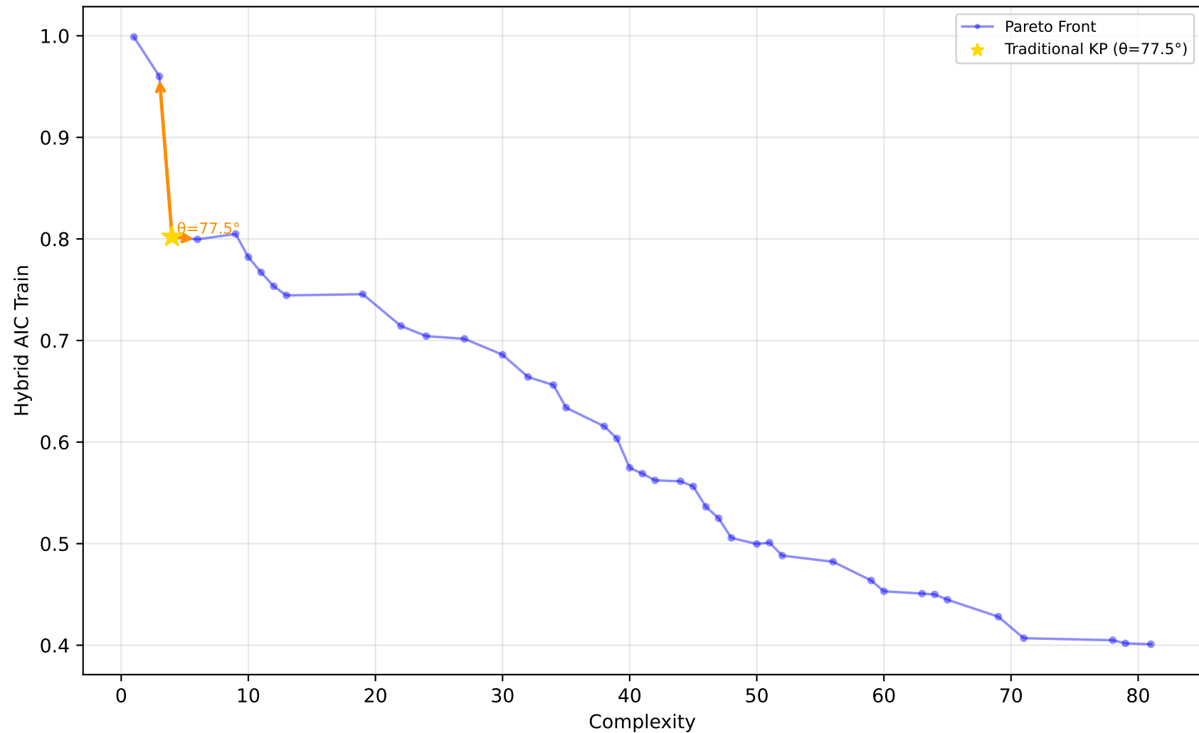
589_fri_c2_1000_25 - Run 19 - SVP - Hybrid AIC Train \lambda_1=0.20, \lambda_2=0.00, \lambda_3=1.00 | Difficulty: 1.00 | Method: hmr
