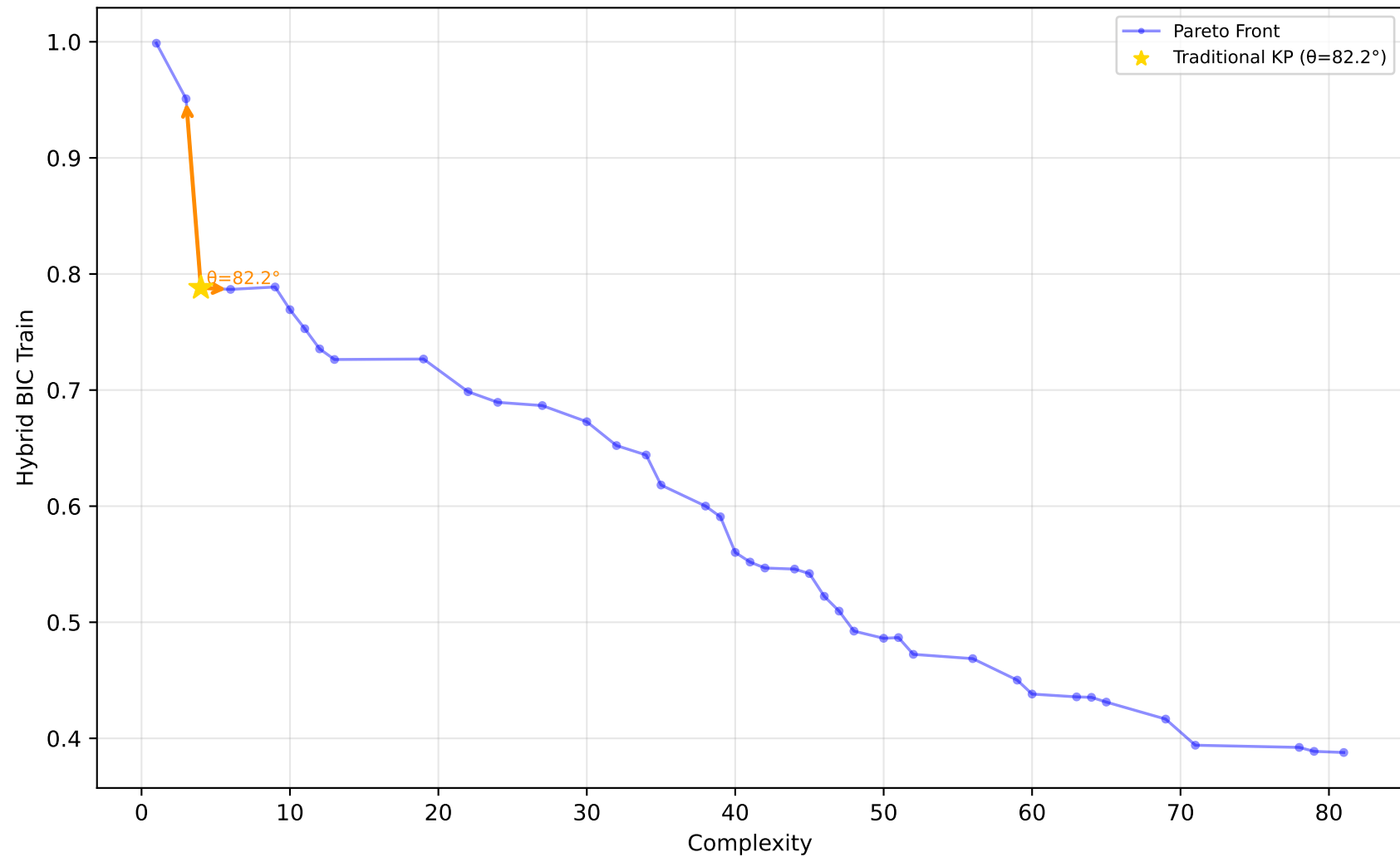
589_fri_c2_1000_25 - Run 19 - SVP - Hybrid BIC Train \lambda_1=0.10, \bar{\lambda}_2=0.00, \bar{\lambda}_3=0.10 | Difficulty: 1.00 | Method: hmr
