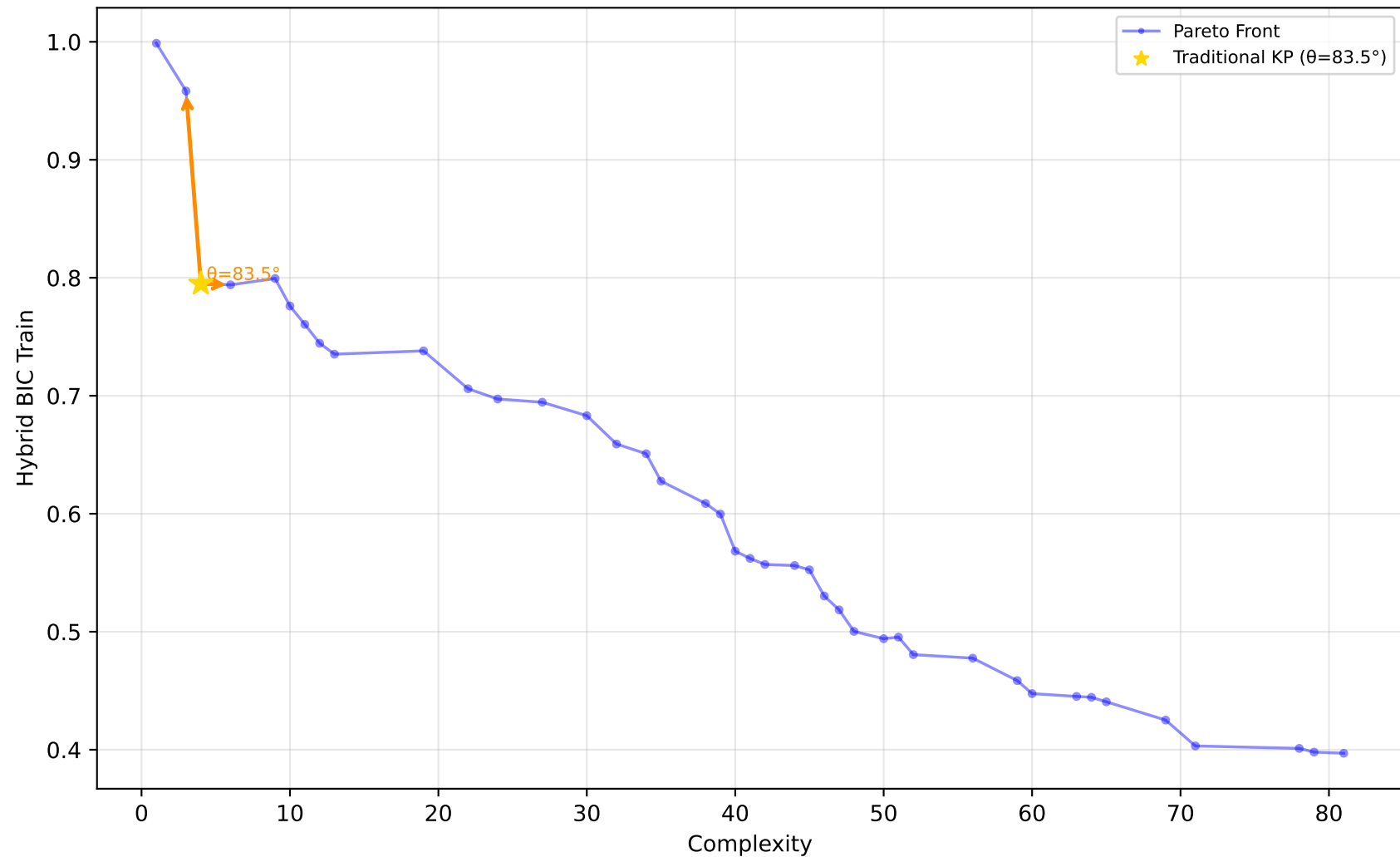
589_fri_c2_1000_25 - Run 19 - SVP - Hybrid BIC Train \lambda_1=0.20, \bar{\lambda}_2=0.00, \bar{\lambda}_3=1.00 | Difficulty: 1.00 | Method: hmr
