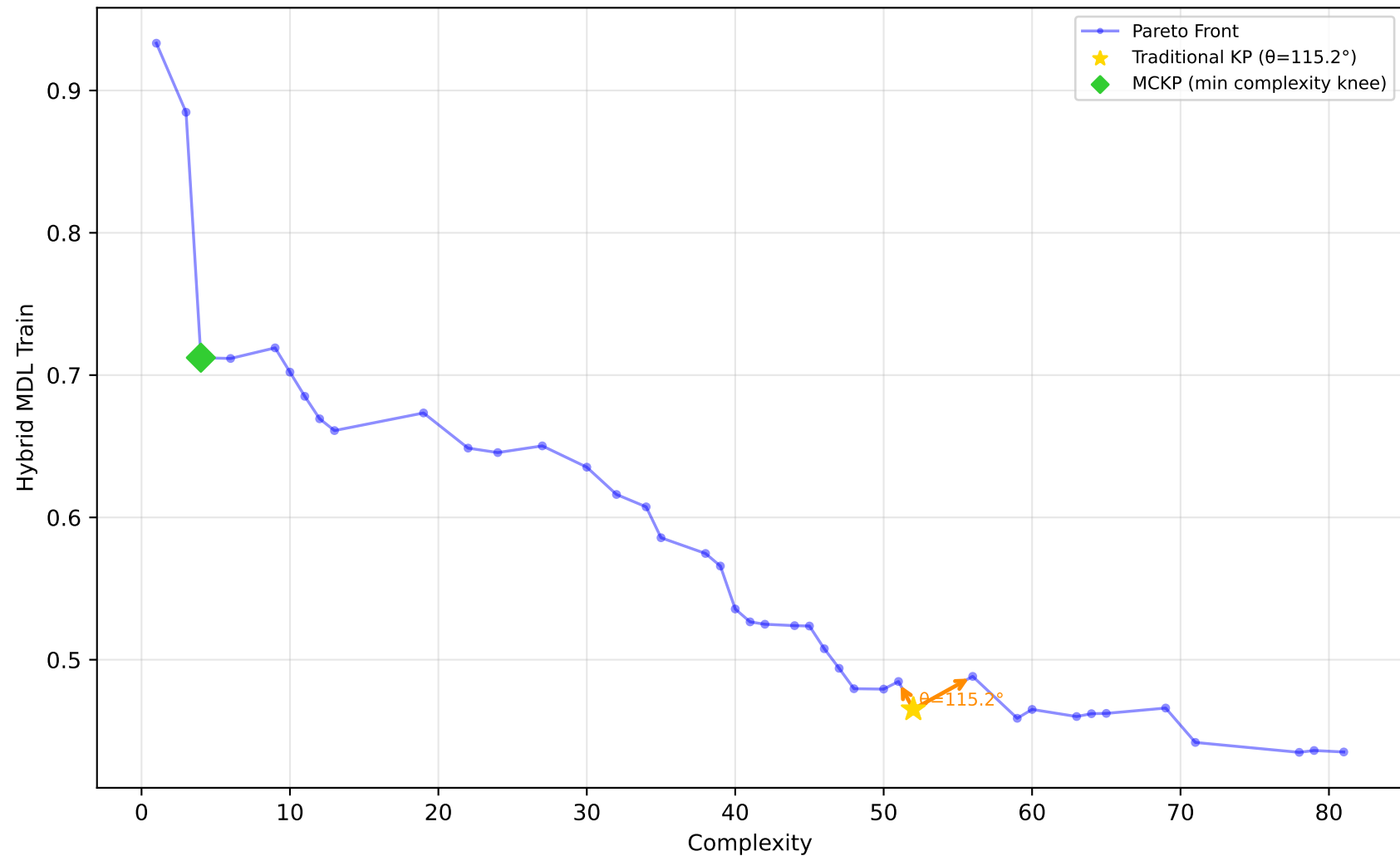
589_fri_c2_1000_25 - Run 19 - SVP - Hybrid MDL Train \lambda_1=0.10, \bar{\lambda}_2=0.00, \bar{\lambda}_3=0.10 | Difficulty: 1.00 | Method: hmr
