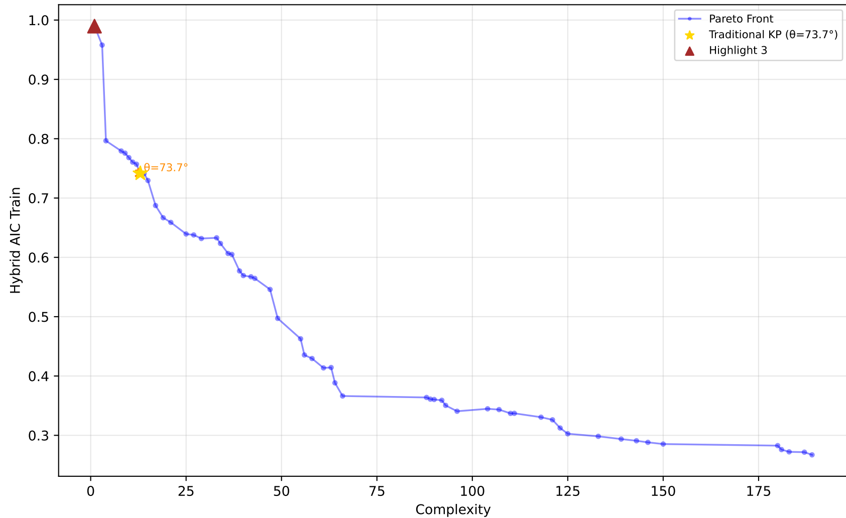
589_fri_c2_1000_25 - Run 1 - MVP - Hybrid AIC Train \lambda_1=0.00, \lambda_2=0.00, \lambda_3=0.00 | Difficulty: 1.00 | Method: hmr
