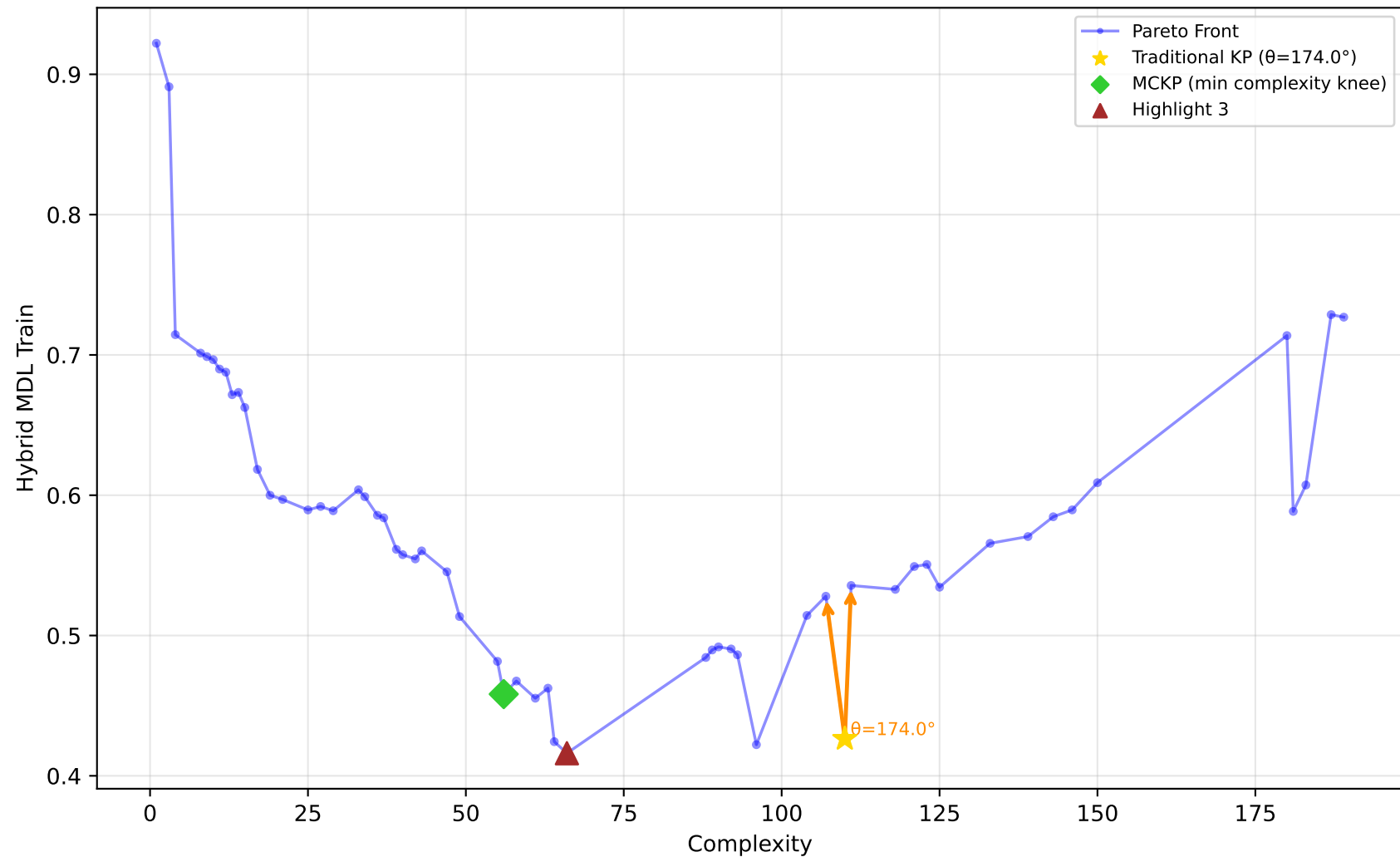
589_fri_c2_1000_25 - Run 1 - MVP - Hybrid MDL Train \lambda_1=0.00, \bar{\lambda}_2=0.00, \bar{\lambda}_3=0.00 | Difficulty: 1.00 | Method: hmr
