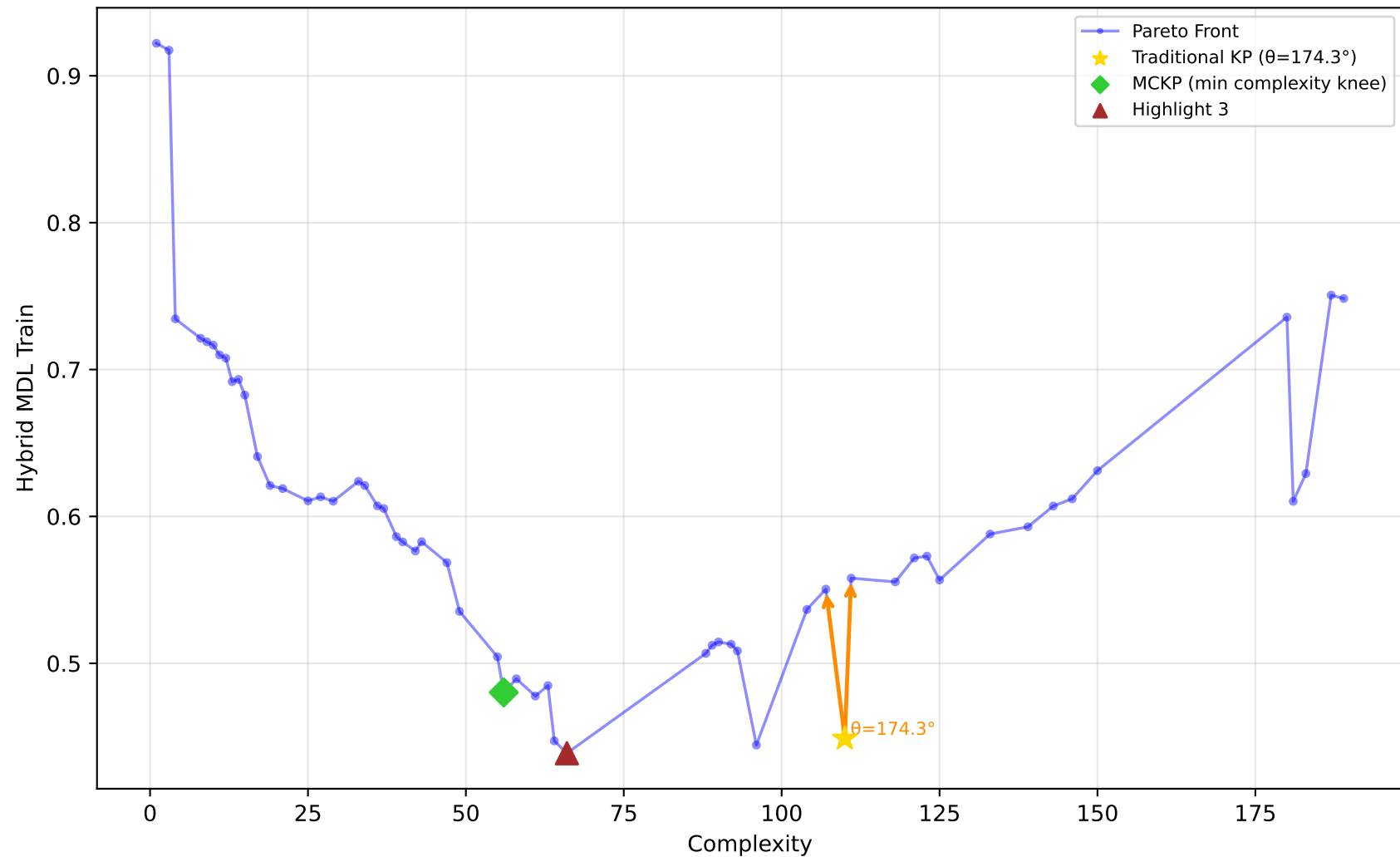
589_fri_c2_1000_25 - Run 1 - MVP - Hybrid MDL Train \lambda_1=0.30, \bar{\lambda}_2=0.00, \bar{\lambda}_3=0.20 | Difficulty: 1.00 | Method: hmr
