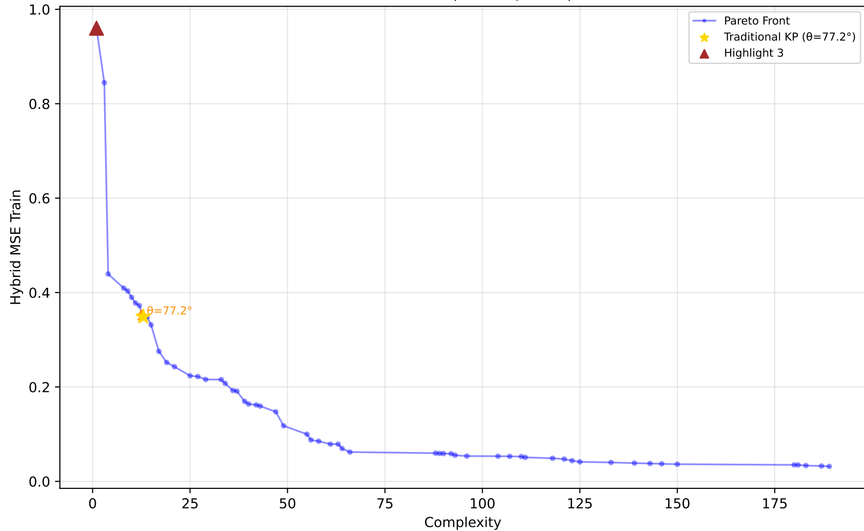
589_fri_c2_1000_25 - Run 1 - MVP - Hybrid MSE Train \lambda_1=0.00, \bar{\lambda}_2=0.00, \bar{\lambda}_3=0.00 | Difficulty: 1.00 | Method: hmr
