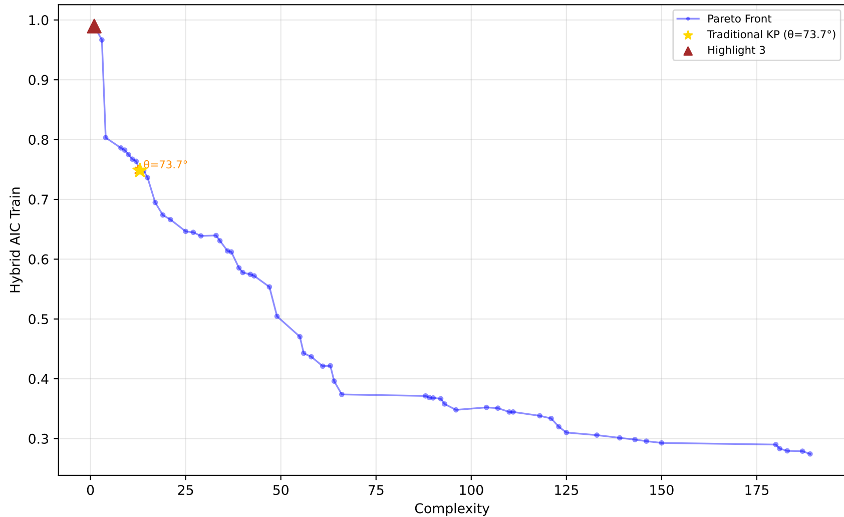
589_fri_c2_1000_25 - Run 1 - SVP - Hybrid AIC Train \lambda_1=0.10, \lambda_2=0.00, \lambda_3=0.10 | Difficulty: 1.00 | Method: hmr
