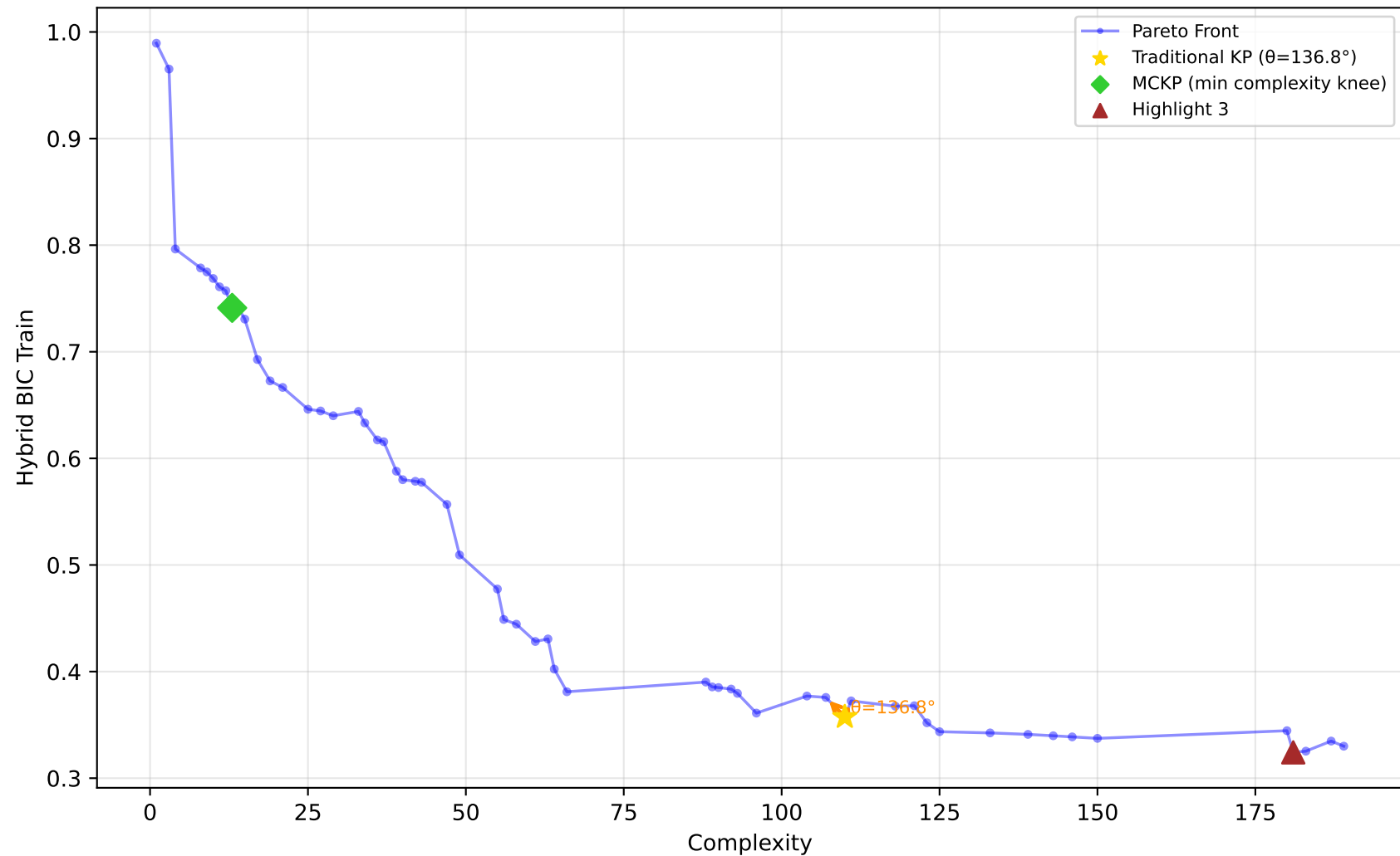
589_fri_c2_1000_25 - Run 1 - SVP - Hybrid BIC Train \lambda_1=0.10, \lambda_2=0.00, \lambda_3=0.10 | Difficulty: 1.00 | Method: hmr
