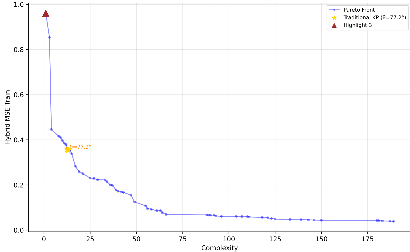
589_fri_c2_1000_25 - Run 1 - SVP - Hybrid MSE Train \lambda_1=0.10, \lambda_2=0.00, \lambda_3=0.10 | Difficulty: 1.00 | Method: hmr
