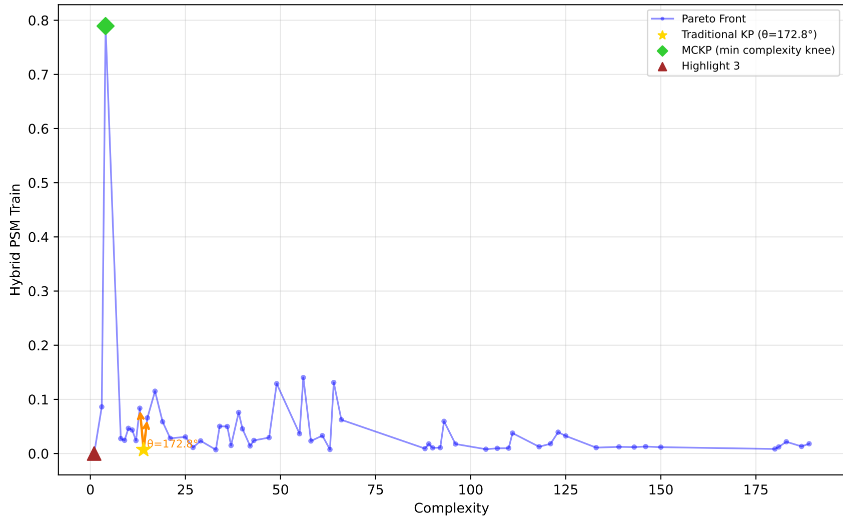
589_fri_c2_1000_25 - Run 1 - SVP - Hybrid PSM Train \lambda_1=0.10, \lambda_2=0.00, \lambda_3=0.10 | Difficulty: 1.00 | Method: hmr
