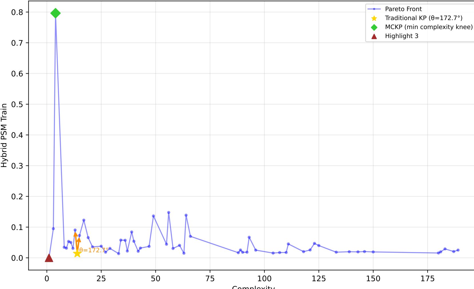
589_fri_c2_1000_25 - Run 1 - SVP - Hybrid PSM Train \lambda_1=0.20 , \lambda_2=0.00 , \lambda_3=1.00 | Difficulty: 1.00 | Method: hmr
