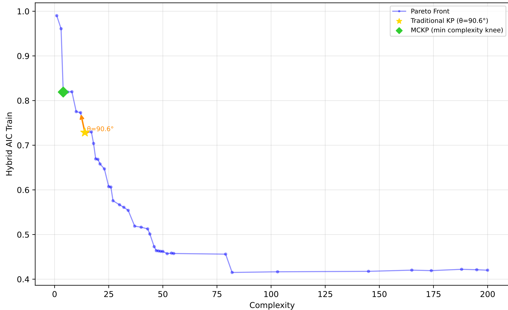
589_fri_c2_1000_25 - Run 20 - MVP - Hybrid AIC Train \lambda_1=0.30, \bar{\lambda}_2=0.00, \bar{\lambda}_3=0.20 | Difficulty: 1.00 | Method: hmr
