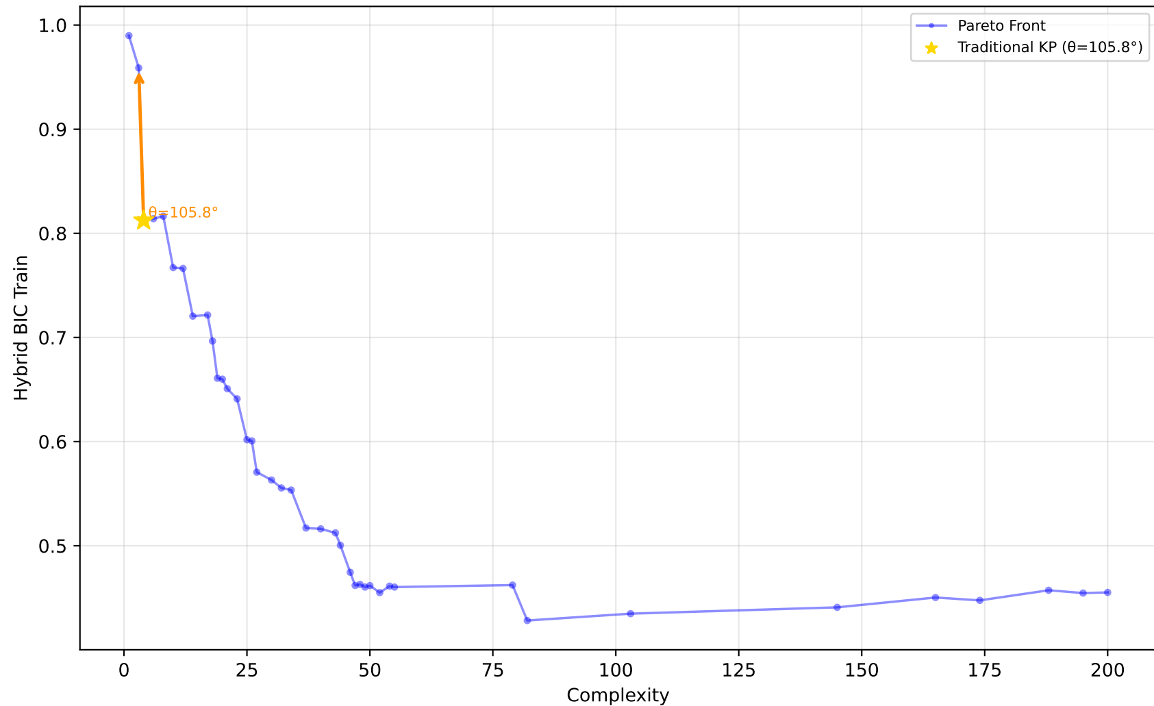
589_fri_c2_1000_25 - Run 20 - MVP - Hybrid BIC Train \lambda_1=0.30, \bar{\lambda}_2=0.00, \bar{\lambda}_3=0.20 | Difficulty: 1.00 | Method: hmr
