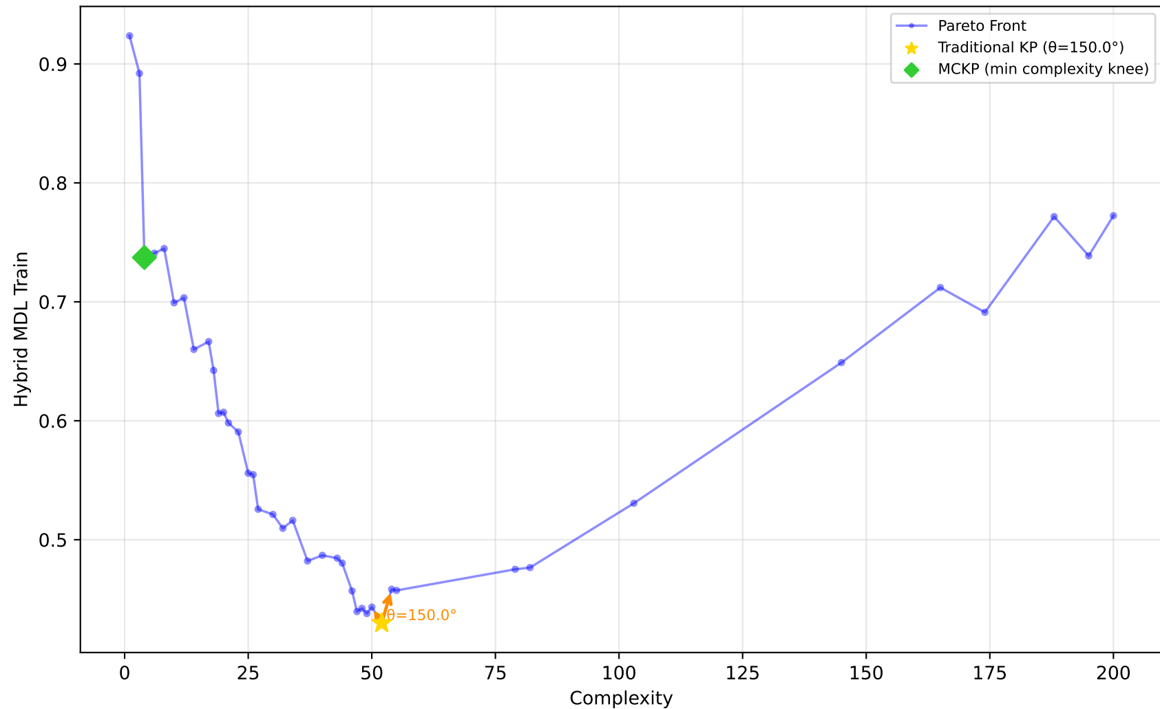
589_fri_c2_1000_25 - Run 20 - MVP - Hybrid MDL Train \lambda_1=0.30, \bar{\lambda}_2=0.00, \bar{\lambda}_3=0.20 | Difficulty: 1.00 | Method: hmr
