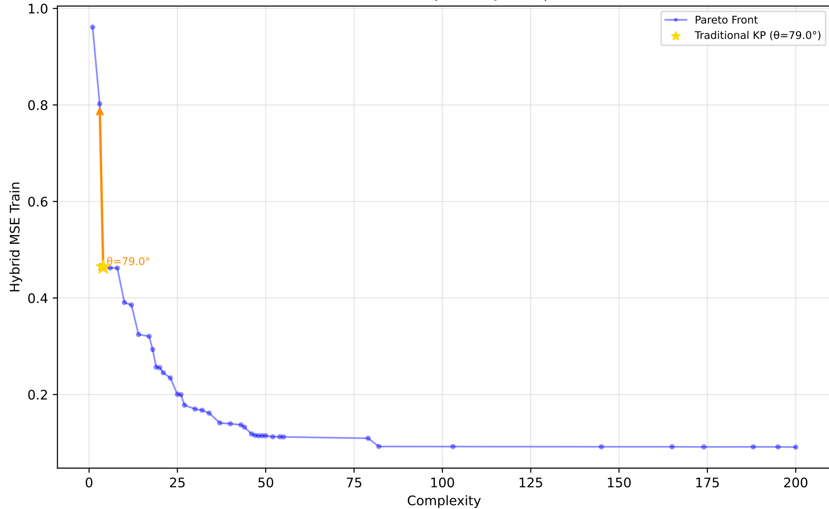
589_fri_c2_1000_25 - Run 20 - MVP - Hybrid MSE Train \lambda_1=0.30, \lambda_2=0.00, \lambda_3=0.20 | Difficulty: 1.00 | Method: hmr
