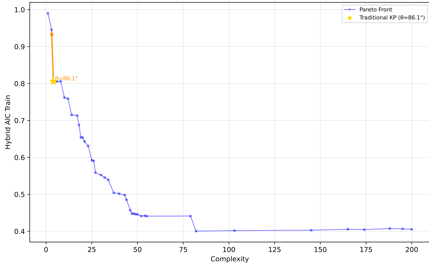
589_fri_c2_1000_25 - Run 20 - SVP - Hybrid AIC Train \lambda_1=0.10, \bar{\lambda}_2=0.00, \bar{\lambda}_3=0.10 | Difficulty: 1.00 | Method: hmr
