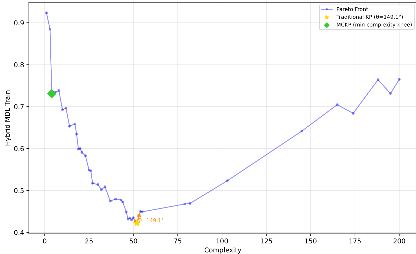
589_fri_c2_1000_25 - Run 20 - SVP - Hybrid MDL Train \lambda_1=0.20, \bar{\lambda}_2=0.00, \bar{\lambda}_3=1.00 | Difficulty: 1.00 | Method: hmr
