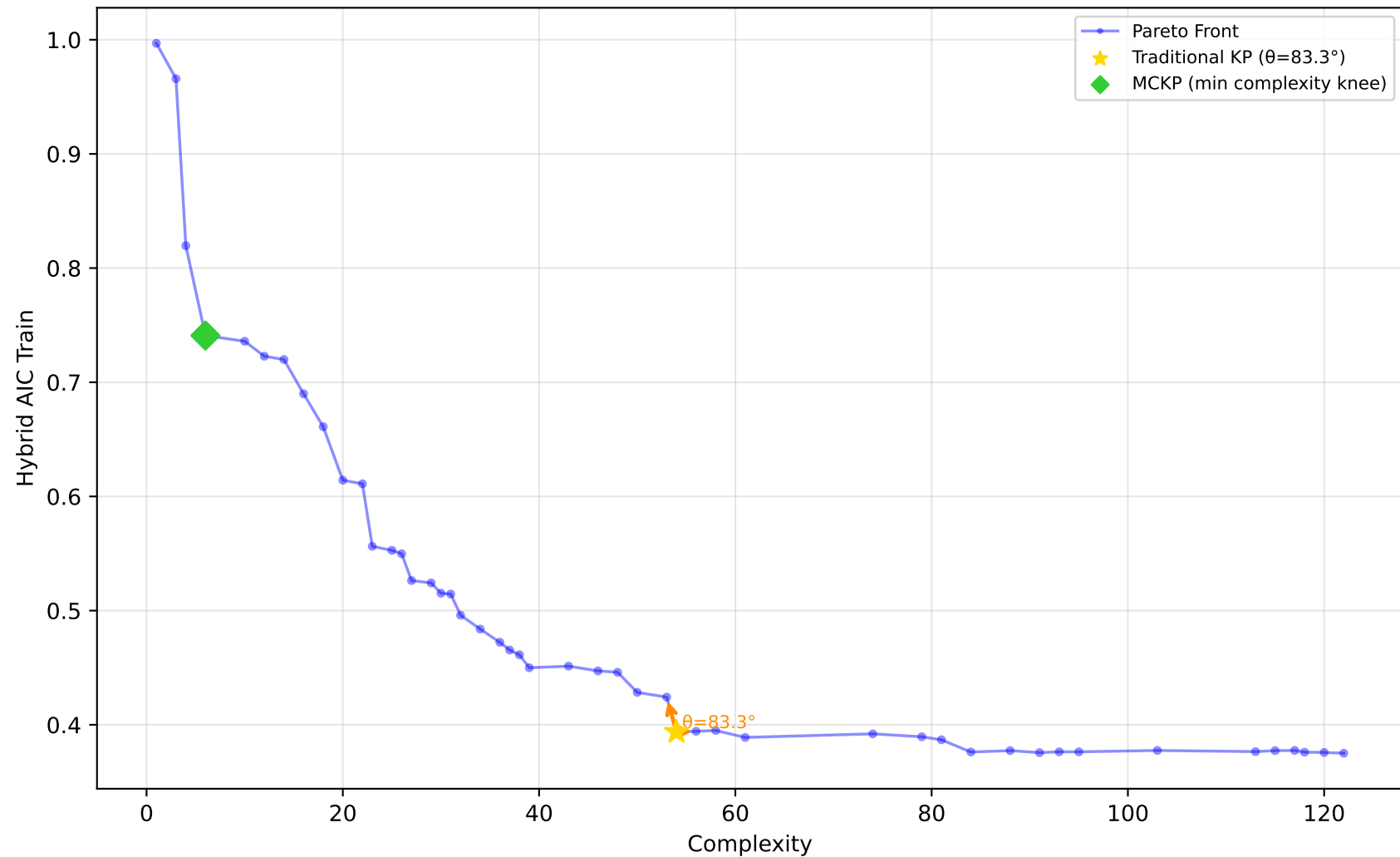
589_fri_c2_1000_25 - Run 21 - MVP - Hybrid AIC Train \lambda_1=0.30, \bar{\lambda}_2=0.00, \bar{\lambda}_3=0.20 | Difficulty: 1.00 | Method: hmr
