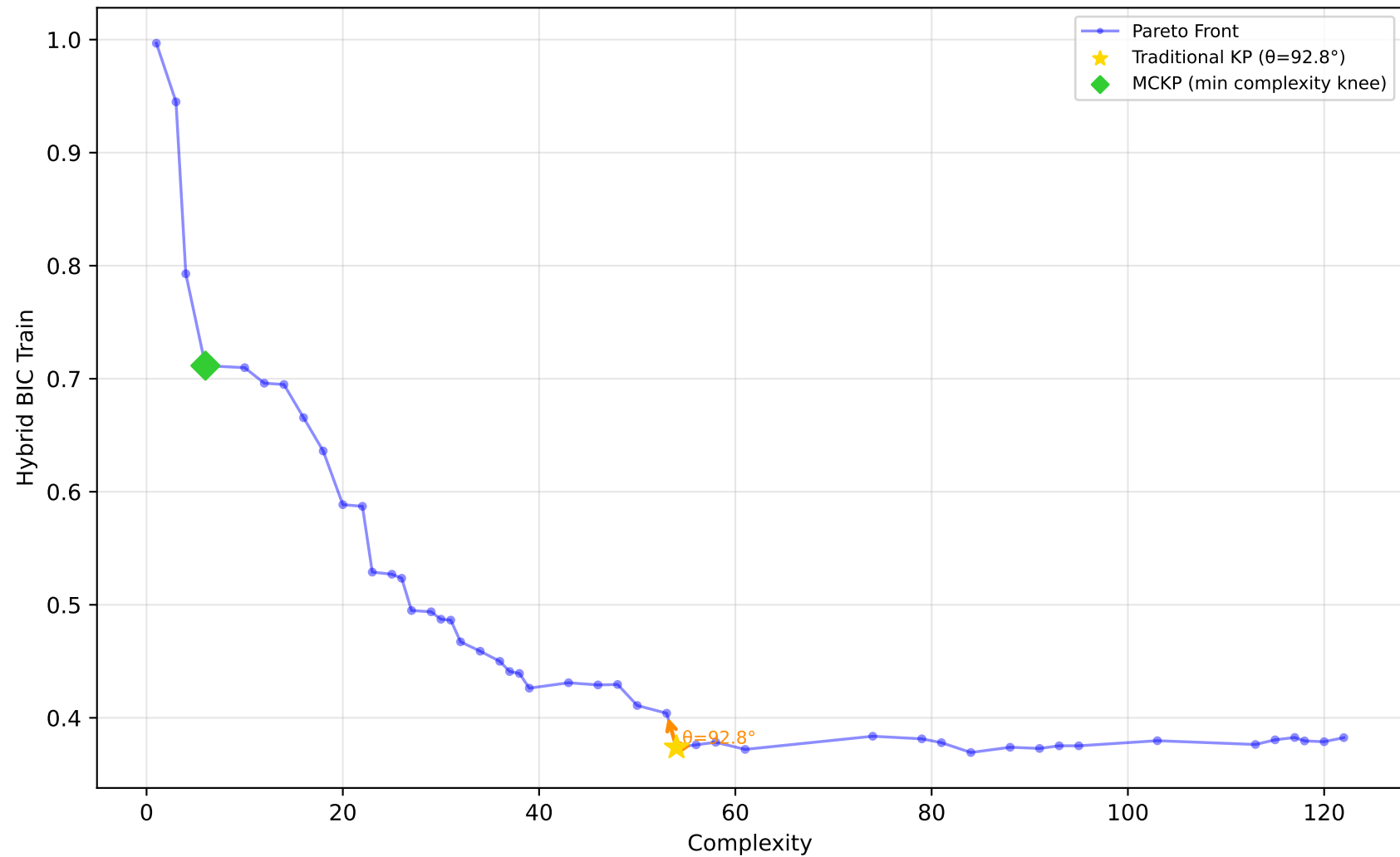
589_fri_c2_1000_25 - Run 21 - MVP - Hybrid BIC Train \lambda_1=0.00, \bar{\lambda}_2=0.00, \bar{\lambda}_3=0.00 | Difficulty: 1.00 | Method: hmr
