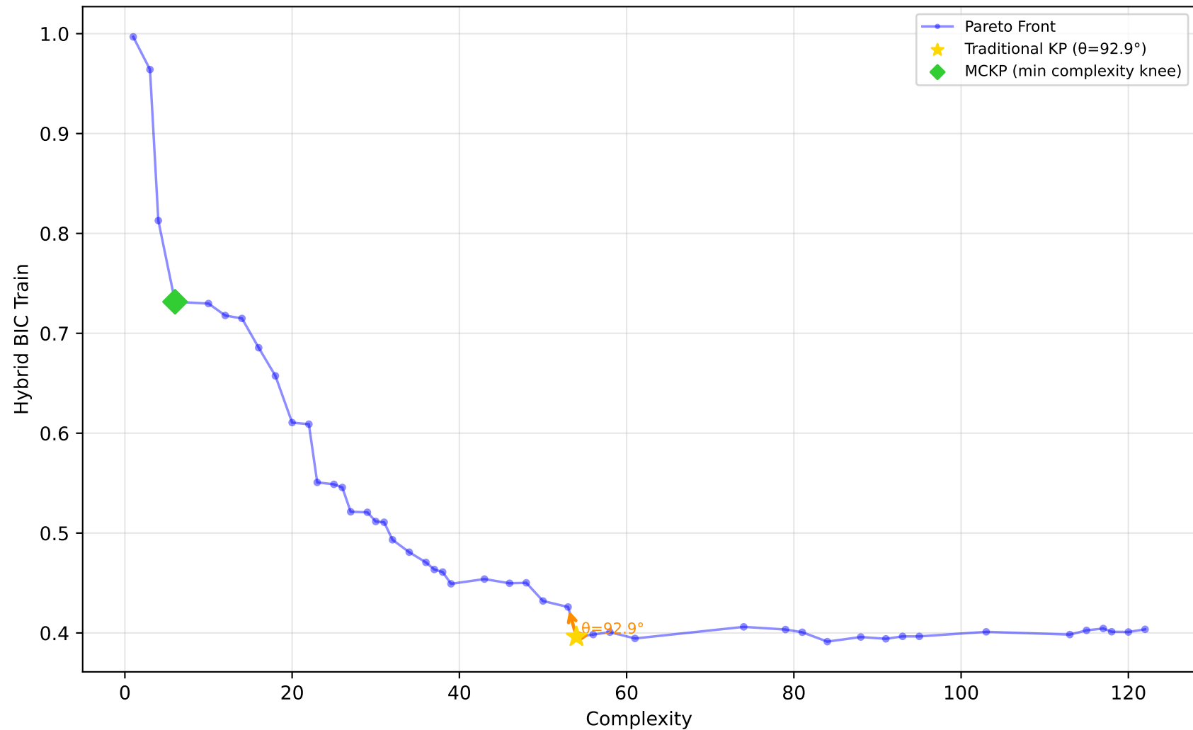
589_fri_c2_1000_25 - Run 21 - MVP - Hybrid BIC Train \lambda_1=0.30, \bar{\lambda}_2=0.00, \bar{\lambda}_3=0.20 | Difficulty: 1.00 | Method: hmr
