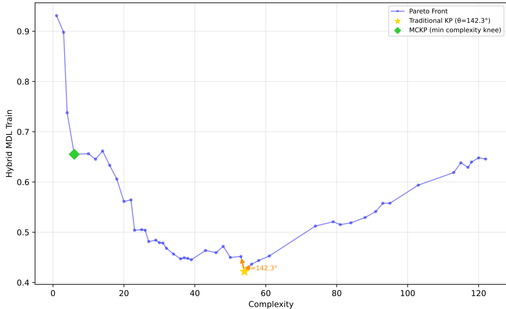
589_fri_c2_1000_25 - Run 21 - MVP - Hybrid MDL Train \lambda_1=0.30, \lambda_2=0.00, \lambda_3=0.20 | Difficulty: 1.00 | Method: hmr
