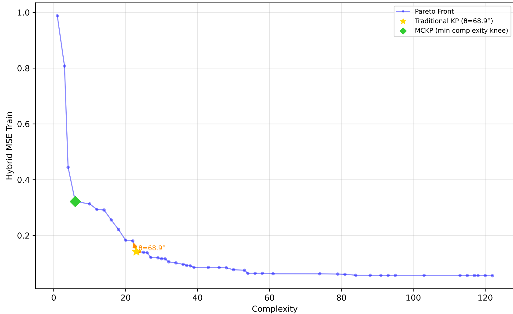
589_fri_c2_1000_25 - Run 21 - MVP - Hybrid MSE Train \lambda_1=0.00, \lambda_2=0.00, \lambda_3=0.00 | Difficulty: 1.00 | Method: hmr
