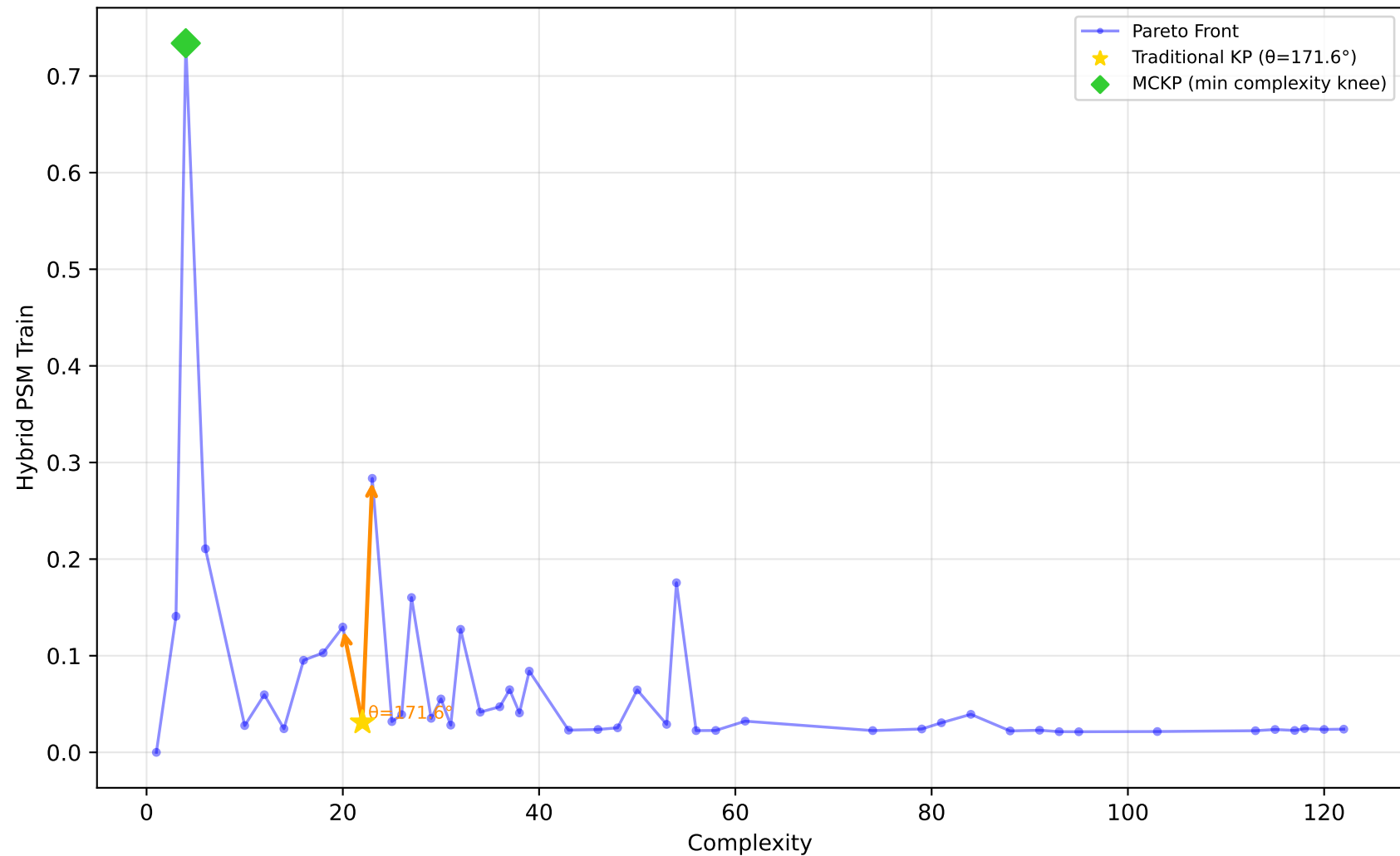
589_fri_c2_1000_25 - Run 21 - MVP - Hybrid PSM Train \lambda_1=0.30, \lambda_2=0.00, \lambda_3=0.20 | Difficulty: 1.00 | Method: hmr
