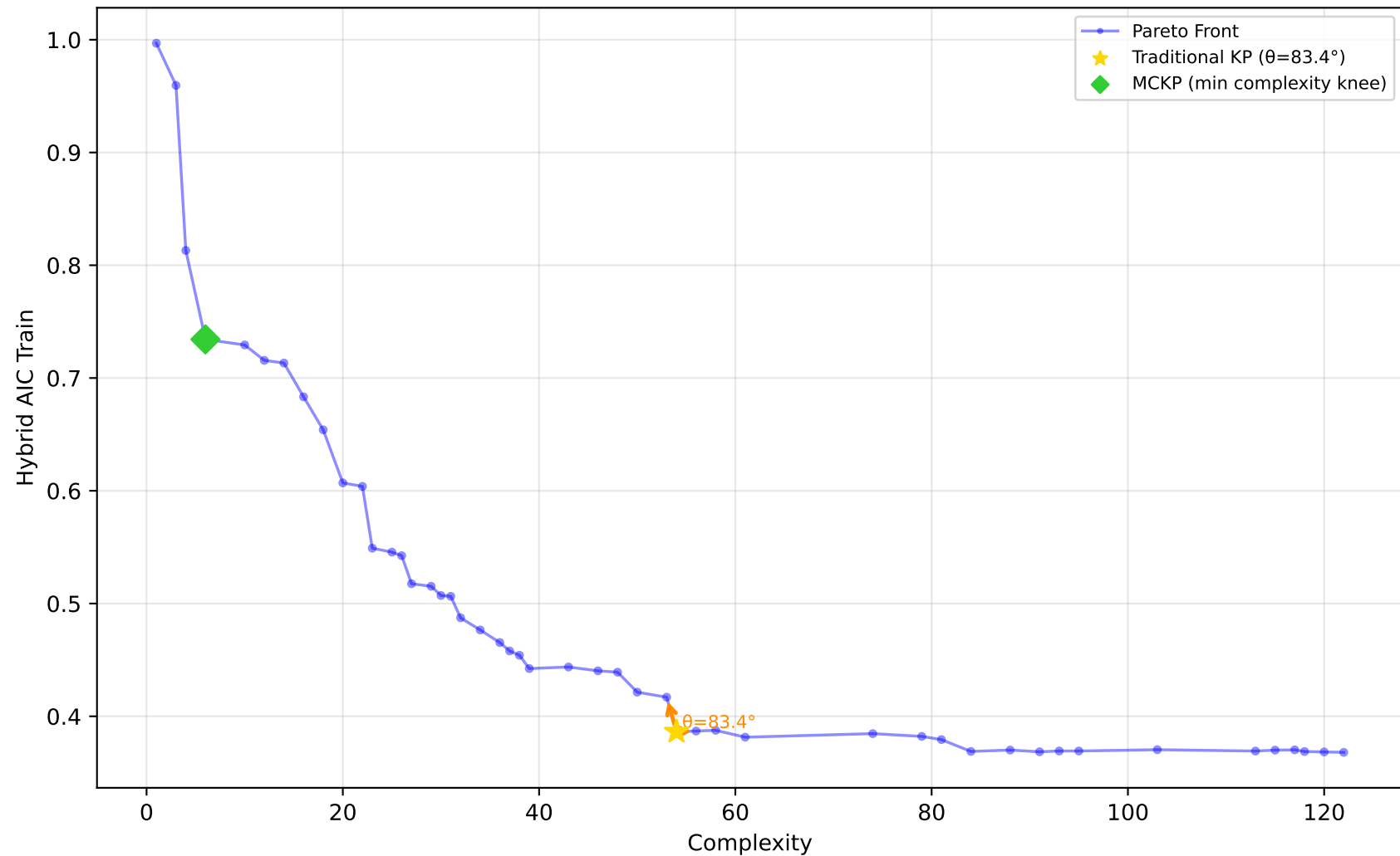
589_fri_c2_1000_25 - Run 21 - SVP - Hybrid AIC Train \lambda_1=0.20 , \bar{\lambda}_2=0.00 , \bar{\lambda}_3=1.00 | Difficulty: 1.00 | Method: hmr
