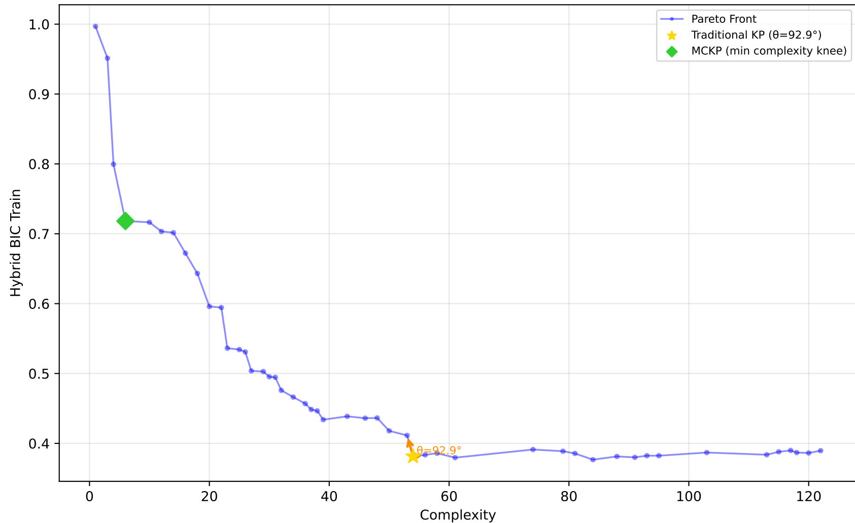
589_fri_c2_1000_25 - Run 21 - SVP - Hybrid BIC Train \lambda_1=0.10, \bar{\lambda}_2=0.00, \bar{\lambda}_3=0.10 | Difficulty: 1.00 | Method: hmr
