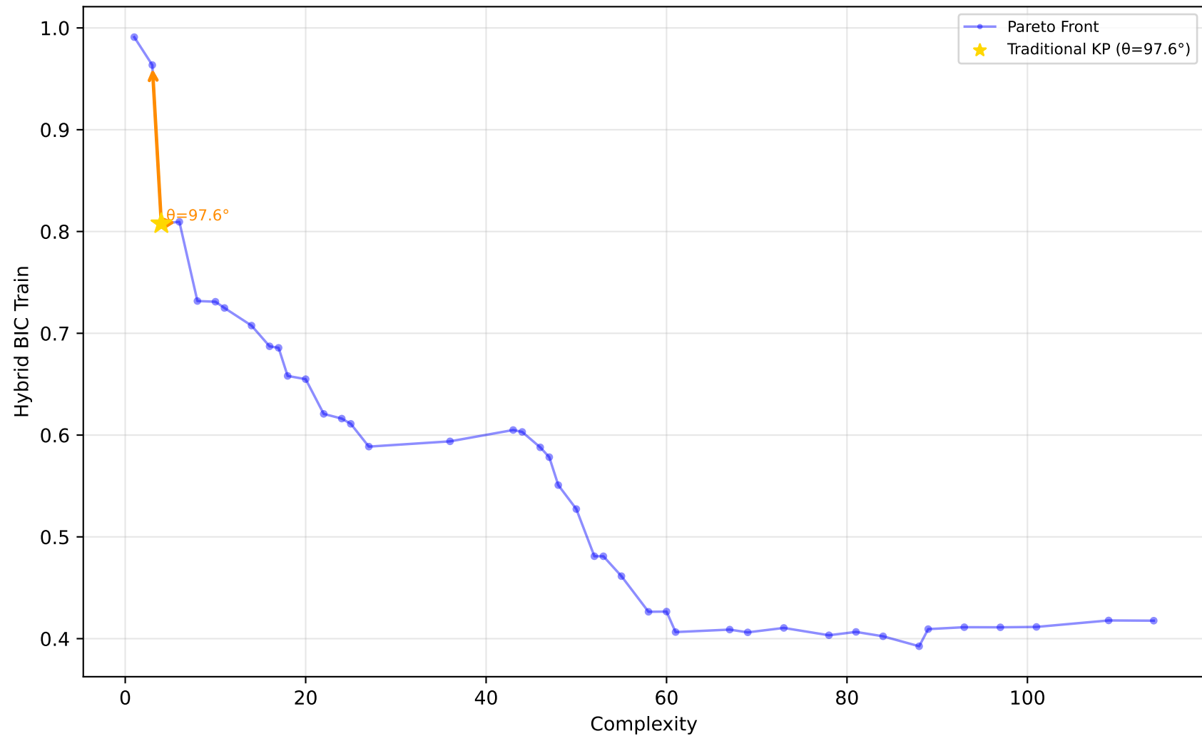
589_fri_c2_1000_25 - Run 22 - MVP - Hybrid BIC Train \lambda_1=0.30, \bar{\lambda}_2=0.00, \bar{\lambda}_3=0.20 | Difficulty: 1.00 | Method: hmr
